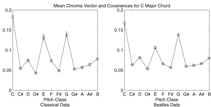
Fig. 6. Mean chroma vector and covariances for C major chord estimated from classical and from the Beatles' data. Because we use diagonal covariance, the variances are shown with "error" bars on each dimension.
