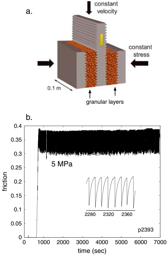
Figure 1. Experimental configuration, with measured data. (a) The biaxial shearing sample, comprised of a three block system with two layers of glass beads. The central block is driven at a constant displacement rate. The stress normal to the layers, applied as indicated by arrows, is maintained constant. (b) Complete record for a representative experiment showing friction \mu \left[\mu = \frac{F/A}{\sigma}\right] versus time, where \sigma is normal load, A is the block area and F is the applied shearing force. The data show hundreds of stick-slip events, with maximum friction of \sim 0.38 and friction drops of \sim 0.08 . The inset shows an expanded view of the friction behavior. The shear rate was initially 10 \mu\text{m/s} for the range 0 to \sim 5000 \mu\text{m} and 5 \mu\text{m/s} thereafter.
