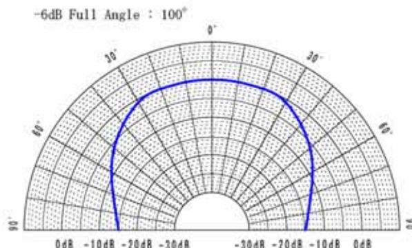
Figure 4. Directivity of a single ultrasonic transducer element. (T4010A: Nippon Ceramic Co.Ltd)
