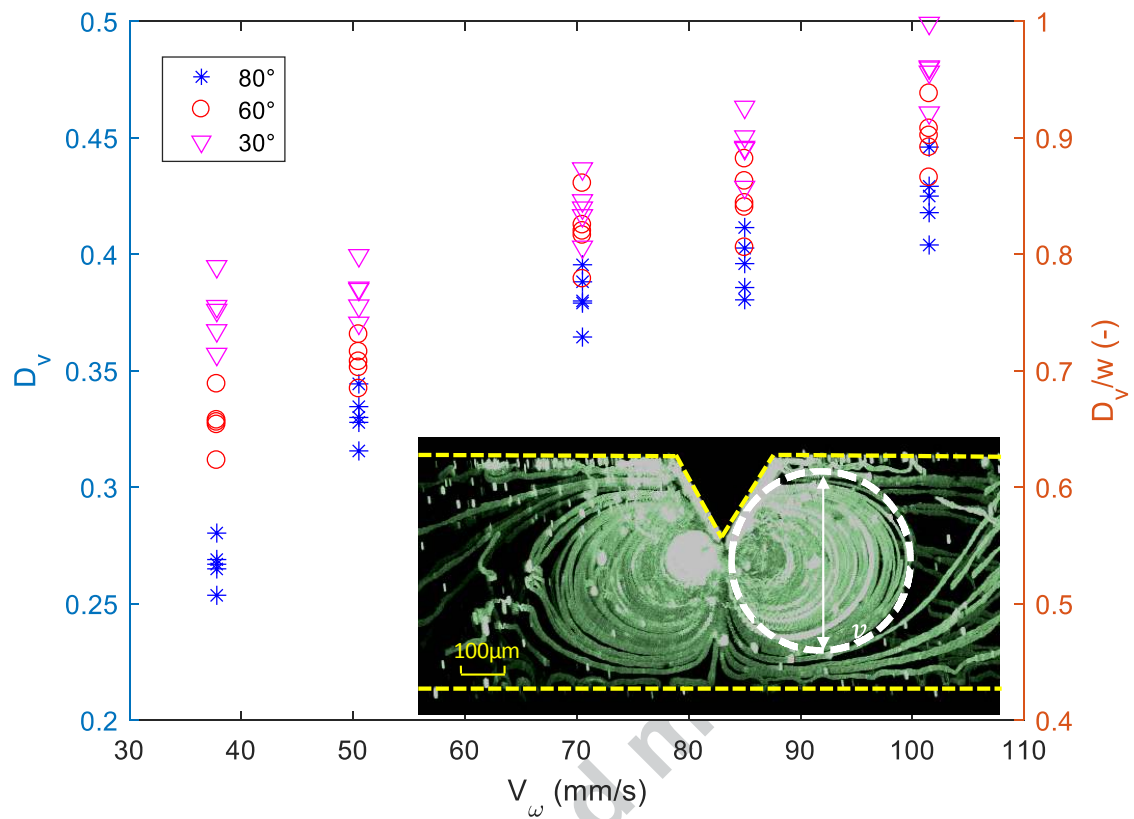
Figure 10: Vortex size D_v and its relative value to the channel width D_v/w at zero flowrate around different sharp edge angles and acoustic stimulations
