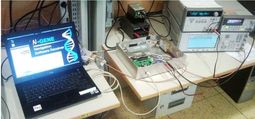
Fig. 3. Picture of the experimental setup (including the laptop for the raw data storage, the discrete component front-end, the power supply and the local oscillators) [own photo]
