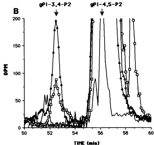
FIG. 3. Identification of polyphosphoinositides produced by immunoprecipitable PI kinase. NIH 3T3 cells expressing the BCR/ abl oncoprotein were grown to confluence and lysed. PI kinase activity was immunoprecipitated by using monoclonal anti- abl protein antibody as described in the legend to Fig. 1. The PI kinase assay was performed with PI as the substrate in the presence of phosphatidylserine as a carrier. The products were extracted into the organic phase, dried under N_2 , deacylated, and separated by HPLC as described in Materials and Methods. Closed triangles represent the deacylated product of PIP (gPIP) produced by anti- abl protein monoclonal antibody-immunoprecipitable PI kinase from quiescent cells which express the BCR/ abl protein. The solid line represents the deacylated [ ^3H ]PI-4-P standard (NEN) coinjected with the sample.
