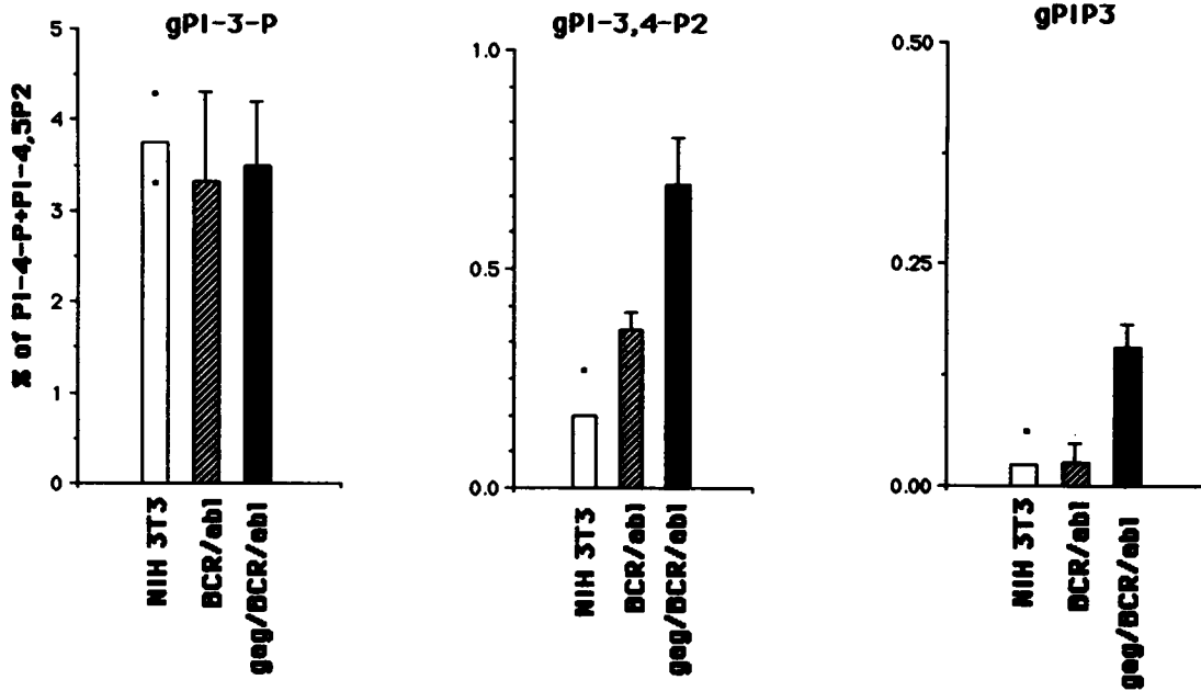
FIG. 5. Total 32 P incorporated into D-3-phosphorylated phosphoinositides in control and transfected NIH 3T3 cells. The total 32 P incorporated into D-3-phosphorylated polyphosphoinositides is expressed as the percentage of 32 PO 4 3- incorporated into PI-4-P plus PI-4,5-P 2 . Symbols: □, results obtained from control NIH 3T3 cells (average of two experiments; the individual results are represented by black dots); ▨, results from cells expressing BCR/abl protein (three experiments; error bars are the standard deviations); ■, results from cells expressing gag/BCR/abl protein (four experiments; error bars are the standard deviations).
