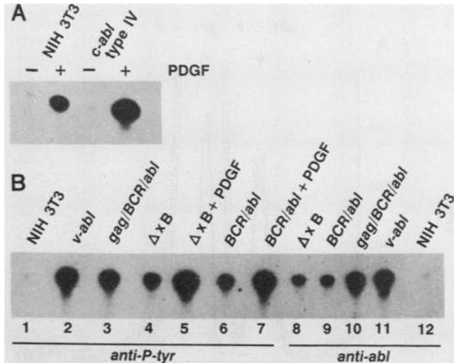
FIG. 1. Association of PI kinase activity with abl proteins. (A) PIP formed by immunoprecipitates from control NIH 3T3 cells (lanes 1 and 2) and cells over expressing c-abl type IV protein (lanes 3 and 4). Cells were grown to confluency in 100-mm plates and brought to quiescence in DMEM supplemented with 1% bovine serum albumin for the last 48 h of culture. A duplicate plate of each cell line was exposed to 10 ng of PDGF-BB per ml for 10 min (lanes 2 and 4). Cells were lysed in a buffer containing 1% Nonidet P-40, and PI kinase was immunoprecipitated by using monoclonal anti-P-Tyr antibody and protein A-Sepharose beads. PI (0.1 mg/ml) was used as the substrate with 0.1 mg of phosphatidylserine per ml as a carrier with 100 \mu M ATP and 20 \mu Ci of [ \gamma - ^{32} P]ATP. The reaction was terminated by addition of 1 N HCl, and the phospholipids were extracted into chloroform-methanol (2:1), dried under N_2 , separated by thin-layer chromatography as described in Materials and Methods, and visualized by autoradiography. The migration position of the newly formed PIP was detected by using nonradioactive PIP which was run in parallel with the samples and visualized by exposure to iodine vapors. (B) PIP formed in immunoprecipitates from whole-cell lysates obtained from control NIH 3T3 cells (lanes 1 and 12) and cells expressing v-abl (lanes 2 and 11), gag/BCR/abl (lanes 3 and 10), \Delta \times B (lanes 4, 5, and 8), and BCR/abl (lanes 6, 7, and 9) proteins. In lanes 5 and 7 cells were exposed to PDGF-BB for 10 min prior to harvest. PI kinase activity was assayed in the immunoprecipitates obtained by using monoclonal anti-P-Tyr (lanes 1 to 7) or monoclonal anti- abl protein (lanes 8 to 12) antibodies. The lipid kinase reaction was performed as described above. The products were separated by thin-layer chromatography and visualized by autoradiography.
