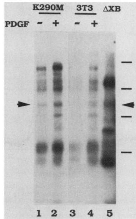
FIG. 2. Detection of an 85-kDa phosphoprotein in immunoprecipitates from cells expressing transforming \Delta \times B protein. Anti-P-Tyr immunoprecipitates from cells overexpressing the K290M tyrosine kinase-inactive mutant protein (lanes 1 and 2), control NIH 3T3 cells (lanes 3 and 4), and anti- abl protein immunoprecipitates from cells expressing transforming \Delta \times B protein (lanes 5 and 6) were washed as described in Materials and Methods and assayed for protein kinase activity in the presence of 5 mM MnCl 2 , 100 \mu M ATP, and [ \gamma - ^{32} P]ATP. After 5 min, the reaction was stopped by the addition of sodium dodecylsulfate (SDS)-containing buffer, and the mixture was heated at 70°C for 5 min. Proteins were resolved by SDS-10% polyacrylamide gel electrophoresis and identified by autoradiography. PDGF-BB (10 \mu g/ml) was added to the cells for 10 min prior to cell lysis as indicated at the top. The lines represent the molecular mass markers at 201, 116, 77, and 46 kDa (Bio-Rad). The 85-kDa phosphoprotein is identified by an arrow.
