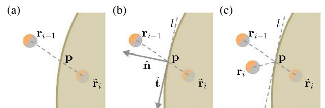
FIG. 23. Numerical implementation of reflective boundary conditions. At each time step, (a) the algorithm checks whether a particle has moved inside an obstacle. If this is the case, (b) the boundary of the obstacle is approximated by its tangent l at the point \mathbf{p} where the particle entered the obstacle and (c) the particle position is reflected on this line. In (b), \hat{\mathbf{t}} and \hat{\mathbf{n}} represent the tangential and normal unitary vectors to the surface at point \mathbf{p} . Note that the orientation of the particle is not flipped.
