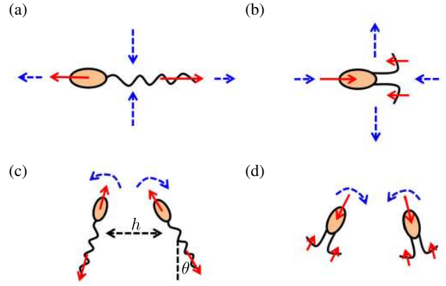
FIG. 9. Flow fields created by swimmers at low Reynolds numbers. (a) Pushers have a positive force dipole ( P > 0 ) and induce an outgoing flow field directed along their swimming direction (repulsion) and an incoming flow field from their sides (attraction). In all panels, the solid red arrows represent the local forcing from the swimmer on the surrounding fluid and the dashed blue arrows represent the fluid flows around the swimmer. (b) Pullers have a negative force dipole ( P < 0 ), inducing an incoming flow field along their swimming direction (repulsion) and an outgoing flow field along their sides (attraction). (c) Two pushers on a converging course reorient each other, tending toward a configuration where they are parallel and swimming side by side ( h is the separation distance between the swimmers, and \theta is the angle between the swimmers direction and the direction normal to their separation). (d) Two pullers on a diverging course reorient each other, tending toward a configuration in which they are antiparallel and swimming away from each other. From Lauga and Powers, 2009.
