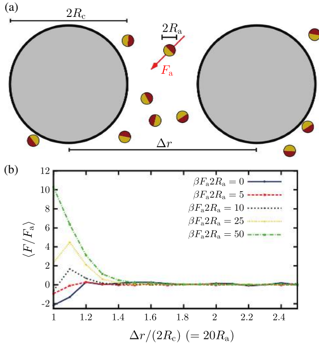
FIG. 21. Emergence of repulsive active-depletion forces in active baths. (a) Schematic representation of two colloidal disks in a bath of active particles. The persistent force F_a acts along a defined axis, which is shown by the arrow as well as the colors, where dark gray (red) corresponds to the back of the particle and light gray (yellow) to its front. (b) Effective rescaled forces \langle F/F_a \rangle experienced by two colloidal disks as a function of their separation for different values of depletant's activity for R_c = 10R_a , where R_c is the radius of the colloids and R_a is the radius of the active particles ( \phi = 0.1 ). Rescaling is applied only as long as \beta F_a 2R_a \neq 0 . Positive values correspond to a repulsion, which dominates any depletion-driven interaction when the bath is active. The larger the active force and the larger the colloid-to-depletant size ratio, the stronger the repulsion. From Harder et al. , 2014.
