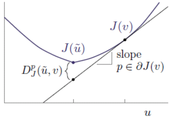
Figure 3. Bregman distance [11]
