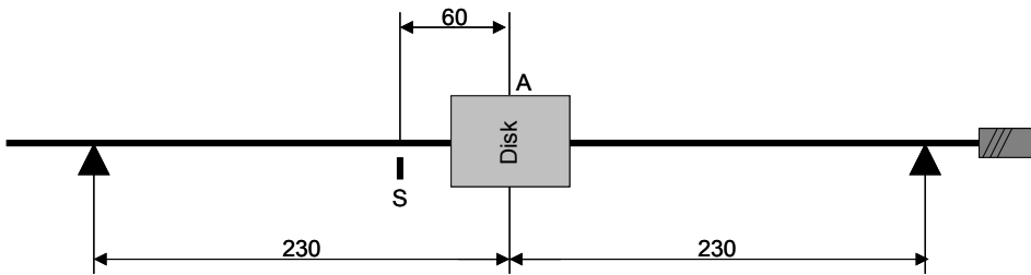
Figure 13. The rotor was driven at the right end. The armature was located at the centre; the radial displacements were measured at the black mark (S). (Dimensions in millimetres).
