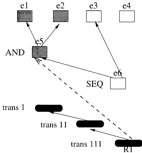
Figure 12. Tracing composite events in Sentinel.
