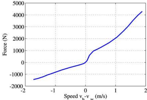
Figure 11. Measured damper characteristic of the passive suspension
