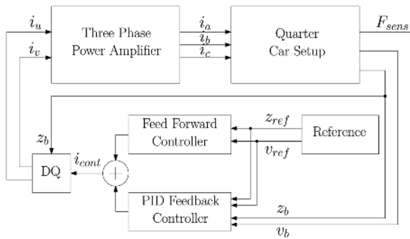
Figure 13. Block diagram of the measurement setup
