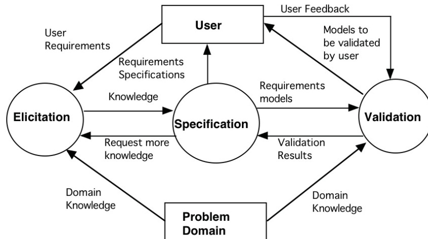
Figure 2: A framework for requirements engineering processes: Loucopoulos and Karakostas (1995) page 21
