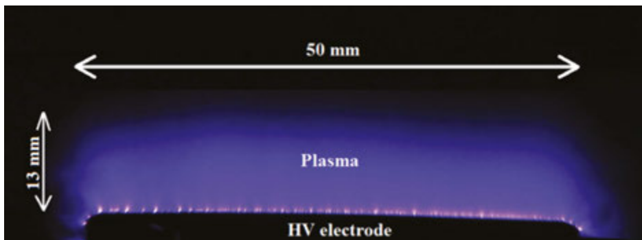
Figure 2. Top view image of SDBD discharge [14].
