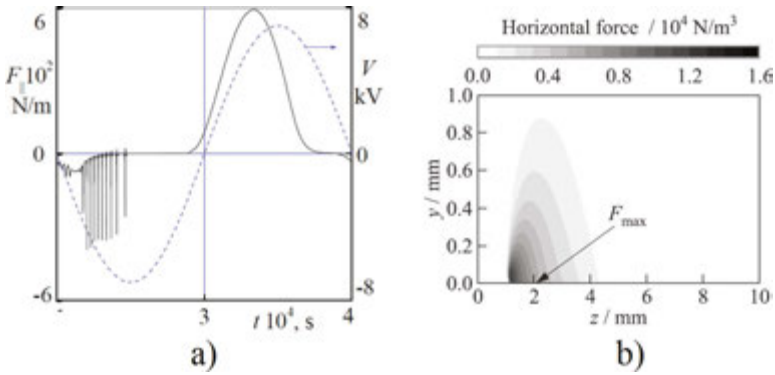
Figure 6. Time evolution of the EHD body force (a) [36], and spatial distribution of the average horizontal force (b) [33].
