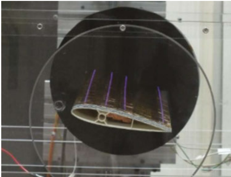
Figure 12. Airfoil equipped with four spanwise plasma actuators [65].
