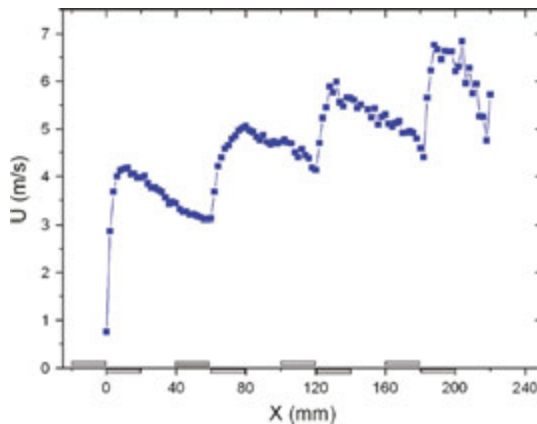
Figure 7. Horizontal velocity profile ( y = 0.5 \text{ mm} ) above four DBD actuators in series [13].
