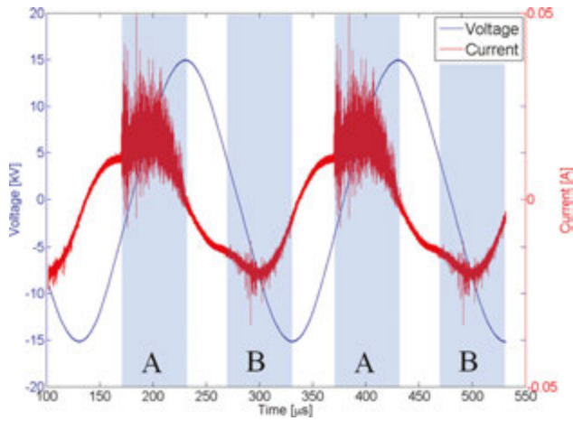
Figure 3. Voltage-current time behavior of a SDBD [15].
