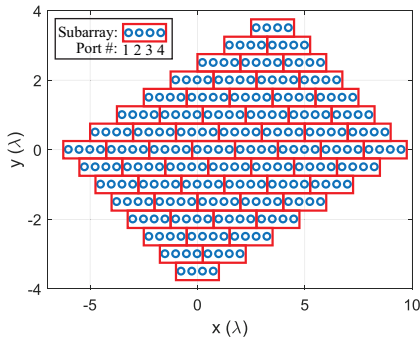
Fig. 4. The proposed AMSPAA layout.
