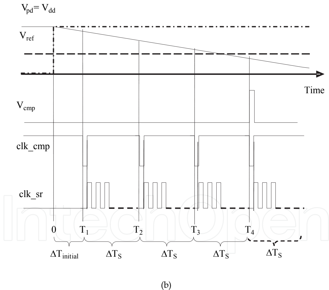
Fig. 7. Architecture's (a) block diagram and (b) control signals
