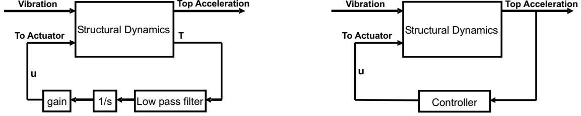
Figure 5. Block Diagram for Tensegrity Vibration Control: Local Integral Force Feedback (left), Acceleration Feedback (right)
