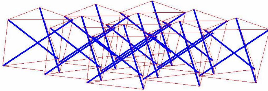
Figure 2. A 9 Stable 3-Bar Units Tensegrity Plate
