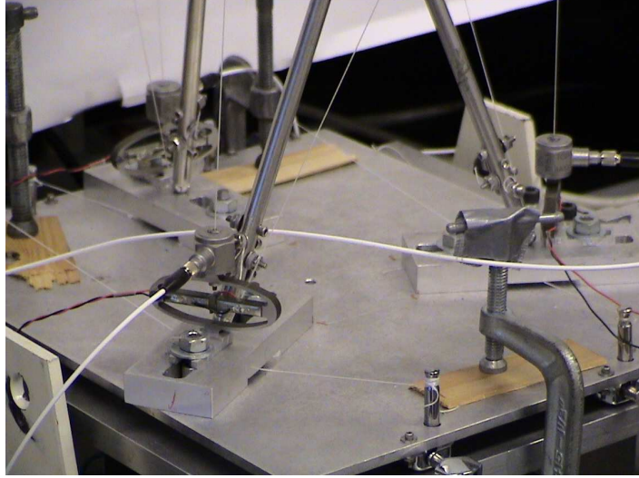
Figure 4. Collocated Sensor and Actuator in the Vertical String
