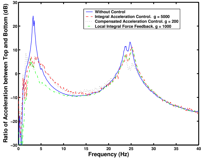
Figure 6. Acceleration Ratio between Top and Bottom Plate (dB) vs Frequency (Hz)
