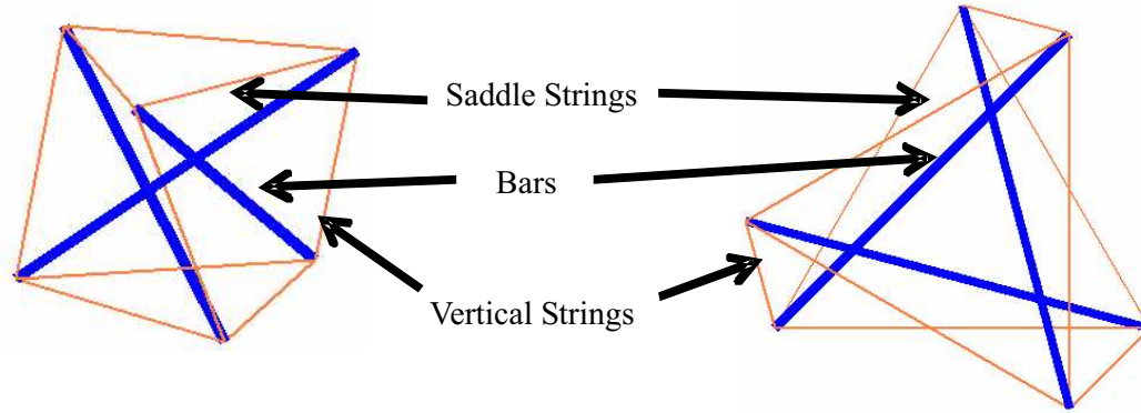
Figure 1. A 3 Dimensional Stable 3-Bar Unit: Perspective View (Left) and Top View (Right)
