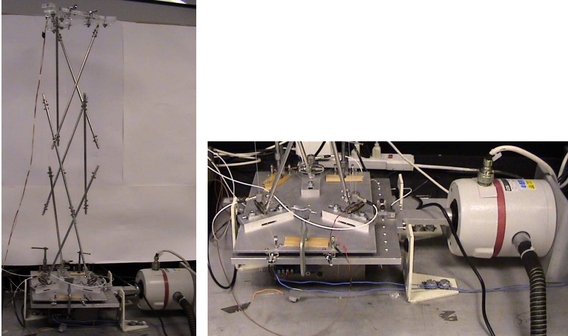
Figure 3. Experimental Setup
