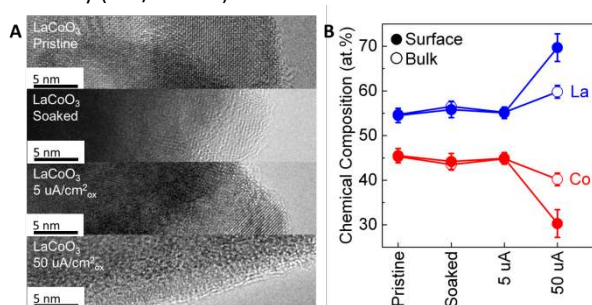
Figure 3. (A) TEM images and (B) EDS-determined chemical compositions of LaCoO 3 in pristine state and operated at 0 (soaking), 5 and 50 \mu\text{A}/\text{cm}^2_{\text{ox}} for 2 h at pH 7. The error bars in (B) represent the standard deviation of multiple spots.
