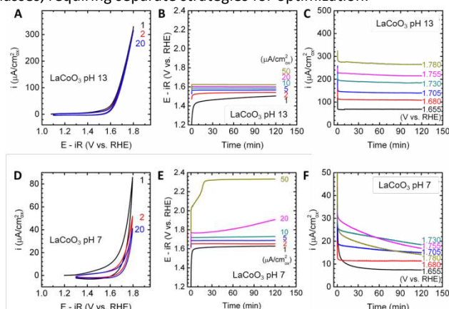
Figure 1. Electrochemical measurements of the \text{LaCoO}_3 OER activity. (A)(D) Cyclic voltammetry. Numbers indicate cycles. (B)(E) Galvanostatic experiments at various current densities. (C)(F) Potentiostatic experiments at various voltages. (A)-(C) was measured in pH 13 electrolyte prepared with 0.1 M KOH, while (D)-(E) was measured in pH 7 electrolyte prepared with 0.4 M \text{NaH}_2\text{PO}_4 , 0.6 M \text{Na}_2\text{SO}_4 and proper amount of NaOH.
