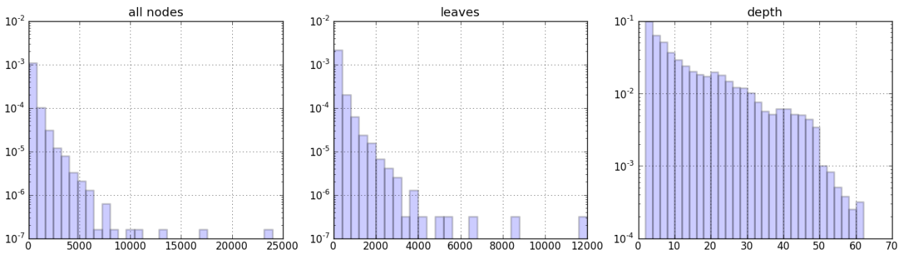
Fig. 12: Histograms of tree sizes, number of leaves, and depths of the trees obtained with our clustering algorithm over all datasets. The median tree is of depth 9, with 33 nodes and 17 leaves, whereas the average is 13 / 324 / 162, meaning that a few trees are much larger than the others.
