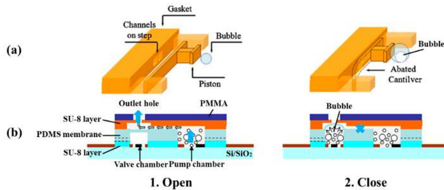
Figure 3. Two types of schematic diagrams of electrochemical actuated microvalves. (a) A microvalve based on electrochemically actuated SU8 cantilever [37]; (b) A microfluidic valve based on electrochemical (ECM) actuated membrane [39].
