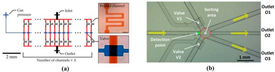
Figure 10. Applications of multiple pneumatic microvalves: (a) Integrated microfluidic device containing 100 microvalves [73]; (b) Micro-droplet sorter with two pneumatic microvalves [80].
