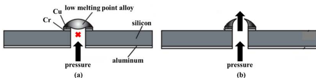
Figure 17. Scheme of the cross-section of the one shot microvalve based on low melting point alloy [105]: (a) In the closed position; (b) In the open position.
