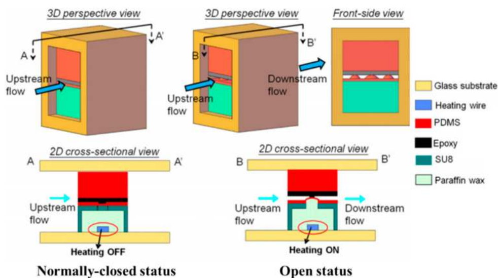
Figure 16. Working principle of the paraffin microvalve [102].
