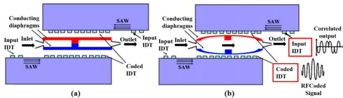
Figure 20. A SAW Microvalve in (a) the OFF/normally closed state; (b) the ON/open state [122].
