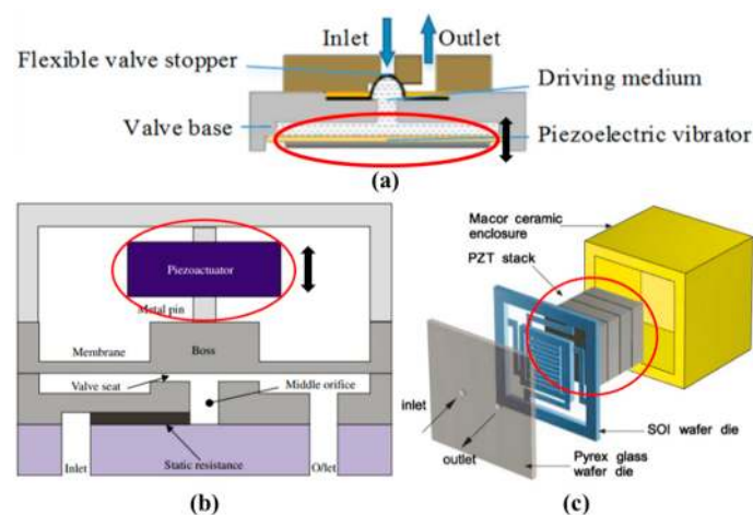
Figure 4. Typical structures of piezoelectric microvalves: (a) a normally-closed piezoelectric microvalve with flexible stopper [40]; (b) a high pressure piezoelectric actuated microvalve [41]; (c) A piezoelectric microvalve for cryogenic applications [42].
