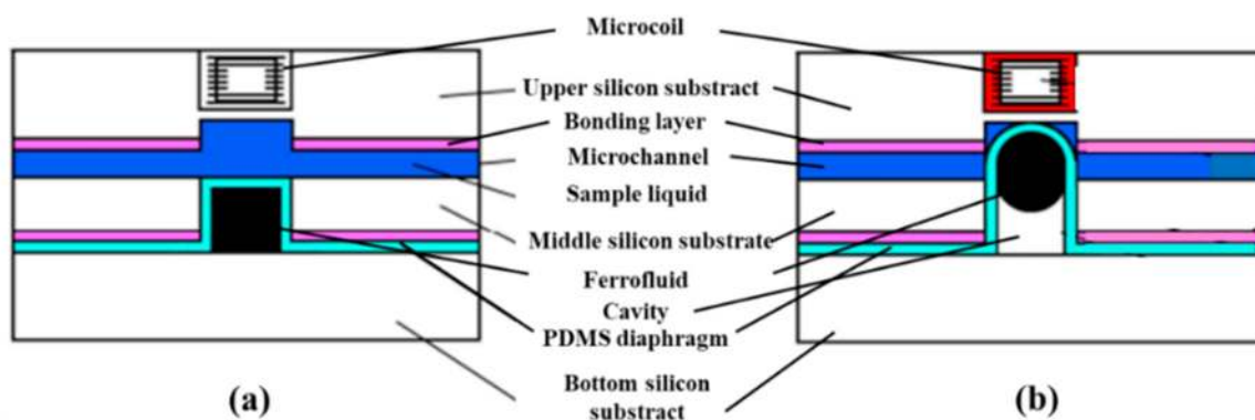
Figure 9. Structure and working principle of microvalve [68]: (a) Open state; (b) Close state.
