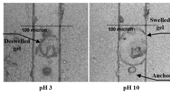
Figure 15. SEM of pH-sensitive microvalve [94].
