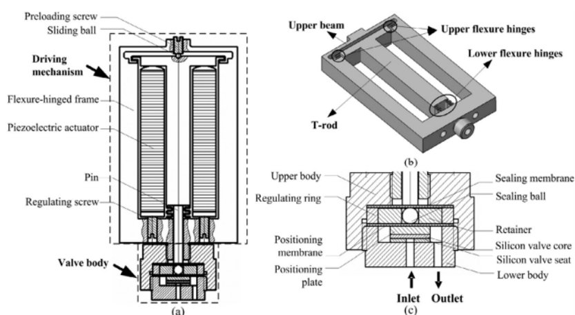
Figure 6. Schematic structure of the microvalve [44]: (a) The structure of the microvalve; (b) The diagram of the 3D geometry model of the frame; (c) The cross-sectional view of the valve body.
