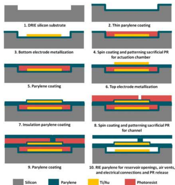
Figure 2. Fabrication process flow of electrostatic actuated microvalve [32].
