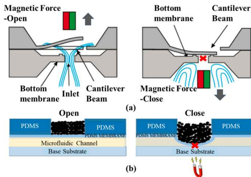
Figure 7. Schematics of two magnetic microvalves: (a) an externally magnetic ON/OFF microvalve [57]; (b) a magnetic microvalve based on MR fluid [58].
