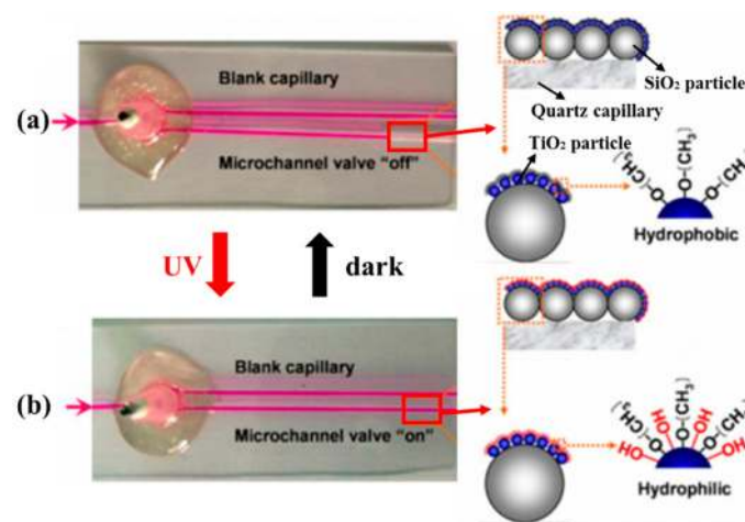
Figure 14. Schematic of UV/dark actuated wettability conversion in the surface of the microvalve [119]: (a) Off status and hydrophobic composite structure before UV irradiation; (b) On status and hydrophilic composite structure after UV irradiation.
