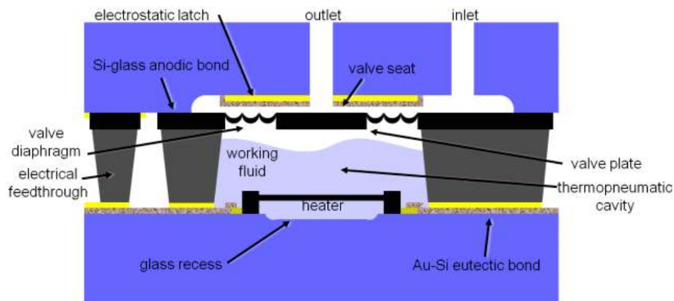
Figure 12. Cross-section view of thermopneumatic microvalve [91].
