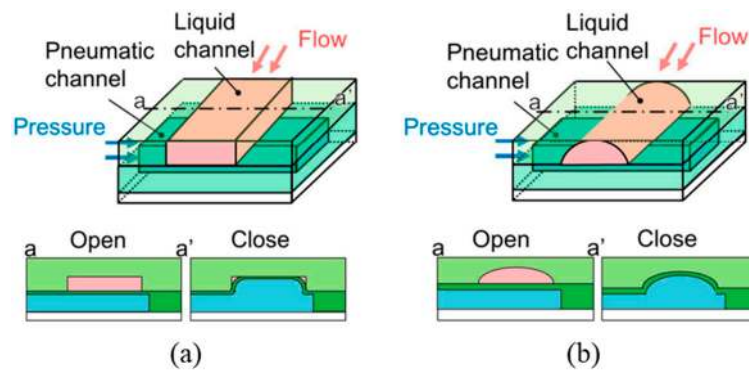
Figure 11. Cross sections of microchannels in pneumatic pressure-driven microvalves [84]: (a) Rectangular cross section; (b) Semicircular cross section.
