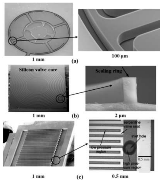
Figure 5. SEM photographs of components in piezoelectric microvalve: (a) the microchannel [43]; (b) the silicon valve core and the sealing ring [44]; (c) the hole with serpentine groove patterns [42].
