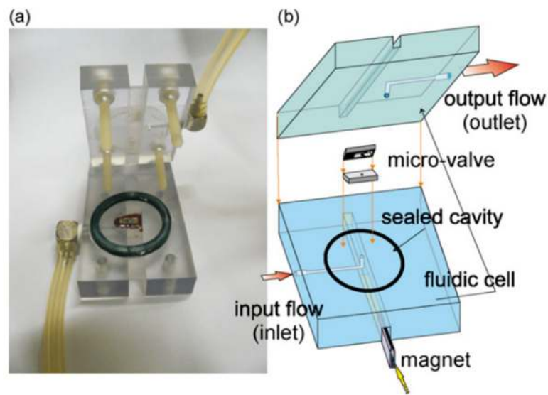
Figure 8. Parts of the magnetic-actuated microvalve and polycarbonate fluidic cell [57]: (a) Experimental set-up; (b) Schematics of the system.
