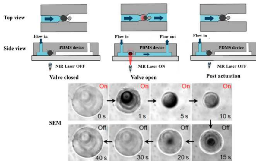
Figure 13. Schematic and SEM of photoresponsive hydrogel microvalve [97].
