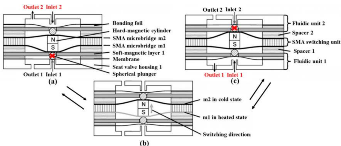
Figure 18. Schematic cross-section of the three-way bistable SMA microvalve [108]: (a) State I; (b) Switching state; (c) State II. (b) Switching from state I to state II is performed by directly heating microbridge m1 with an electrical current.
