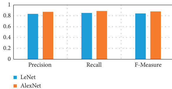
FIGURE 2: Performance comparison of both LeNet-5- and AlexNet-based models in Precision, Recall, and F-Measure.
