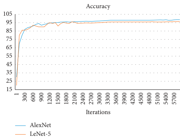
FIGURE 4: Performance comparison of both LeNet-5- and AlexNet-based models in Accuracy at every iteration.
