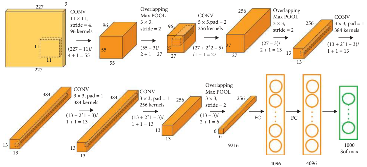
FIGURE 1: Structure of AlexNet model [12].
