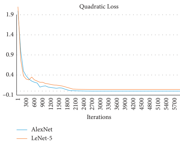
FIGURE 5: Performance comparison of both LeNet-5- and AlexNet-based models in Quadratic Loss at every iteration.
