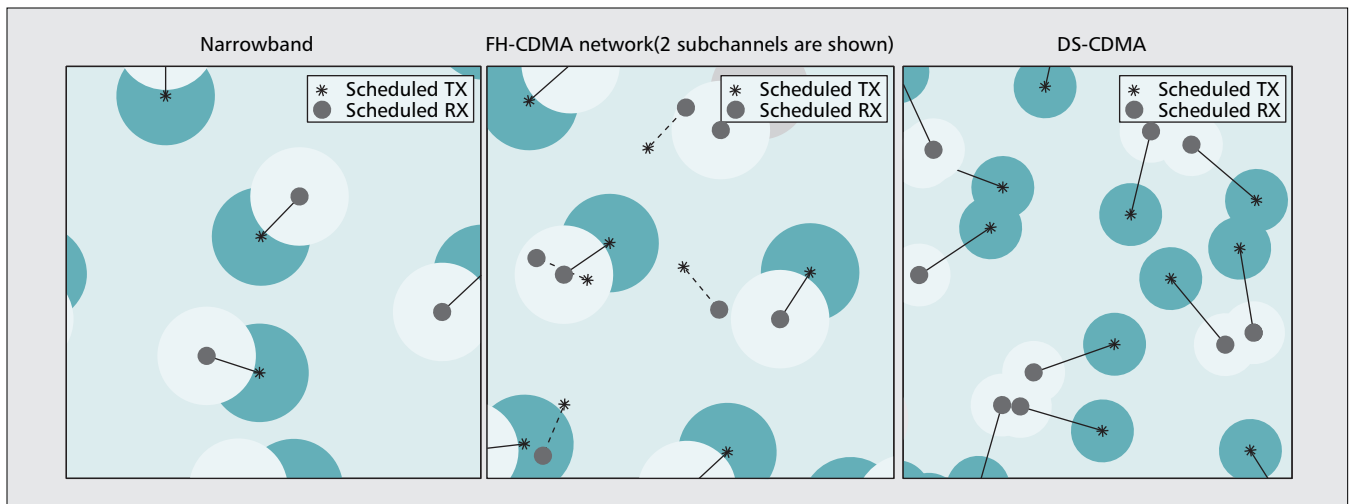
■ Figure 4. Sample transmit/receiver pairs with near-optimal scheduling in narrowband, FH and DS-CDMA networks, from [7]. Narrowband systems require isolated Tx-Rx links. FH (center) allows some colocated links: disks are shown around the users in subband 1, no disks are around users in subband 2. DS throughput is maximized when transmitters and receivers cluster together, as seen at right.
