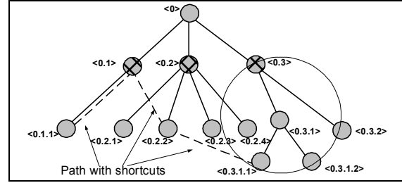
Figure 6: Session path and path shortcuts
