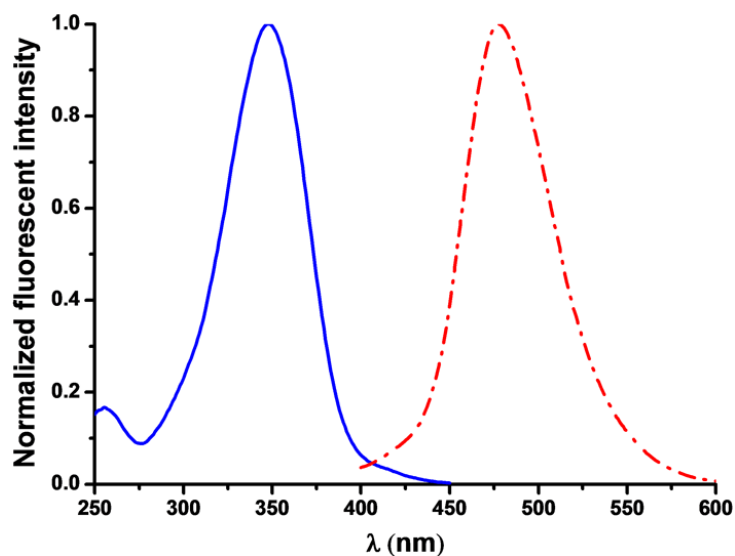
Fig. S1. Normalized excitation ( \lambda_{\text{Ex. max}} = 348 \text{ nm} ) and emission ( \lambda_{\text{Em. max}} = 478 \text{ nm} ) spectra of the aqueous solution of compound 6.
