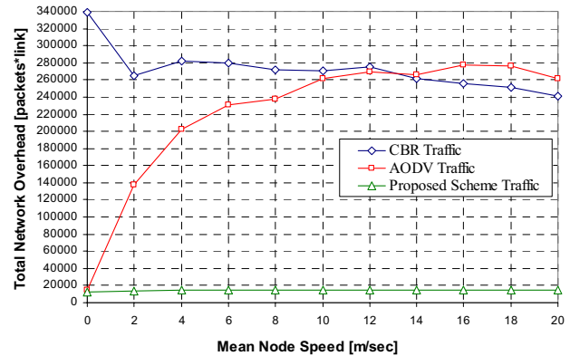
Figure 9. Total Network overhead vs. mean node speed (120 nodes)
