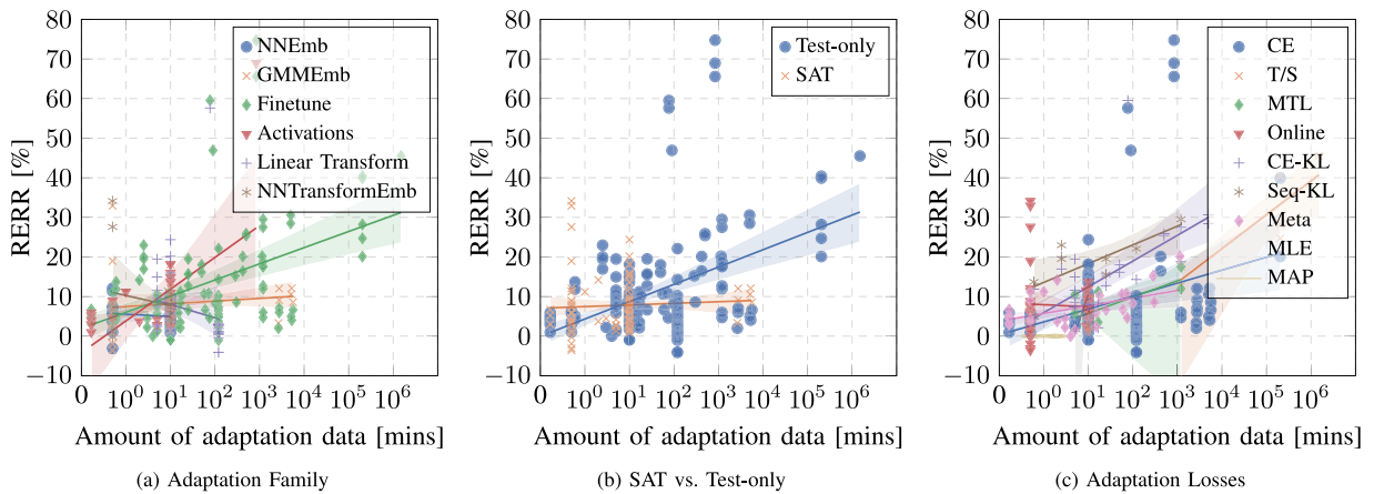
FIGURE 18. Regression analysis for adaptation families, speaker-adaptive training and adaptation losses.
