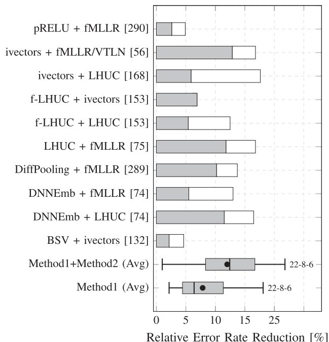
FIGURE 23. Complementarity of selected adaptation techniques.
