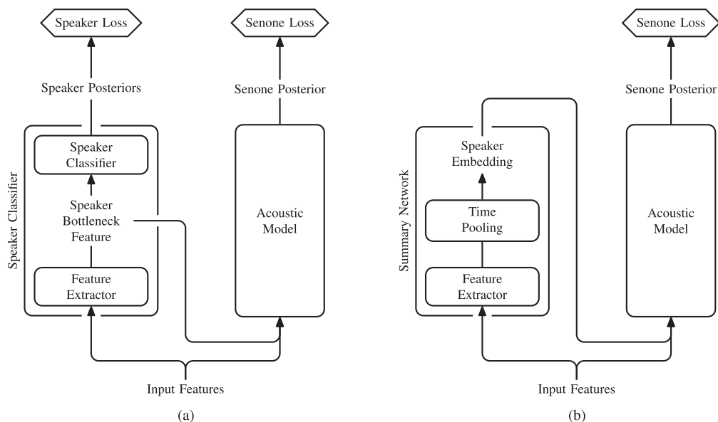
FIGURE 2. (a) Bottleneck feature extraction that uses a pretrained speaker classifier. (b) Summary network extracting speaker embeddings which is trained jointly with the acoustic model.
