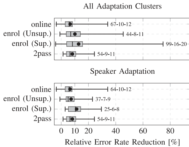
FIGURE 13. Comparison of adaptation results for different adaptation targets: online adaptation, supervised and unsupervised enrollment, and two-pass decoding.
