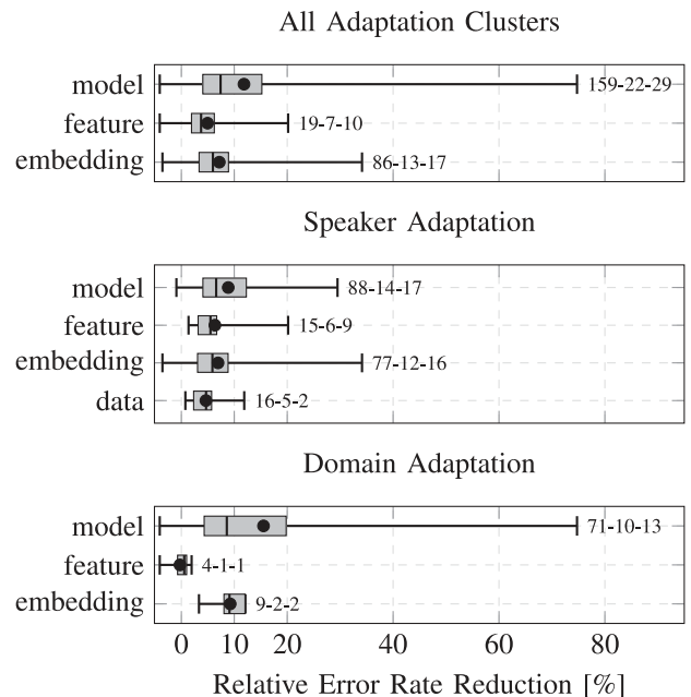
FIGURE 7. Comparison of feature, embedding, and model-level adaptation approaches. Speaker (middle) and domain (bottom) adaptations are based on {utterance, speaker} and {accent, child, domain, disordered} clusters, respectively.
