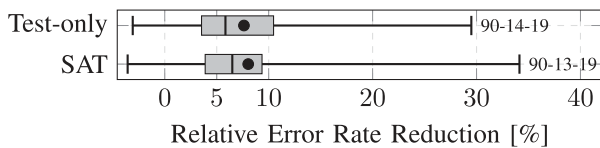
FIGURE 19. Comparison of adaptation results for SAT vs Test-only modes.
