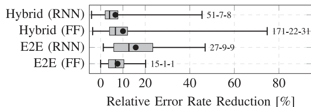
FIGURE 11. Comparison of adaptation results for FF and RNN architectures split by hybrid and E2E systems.
