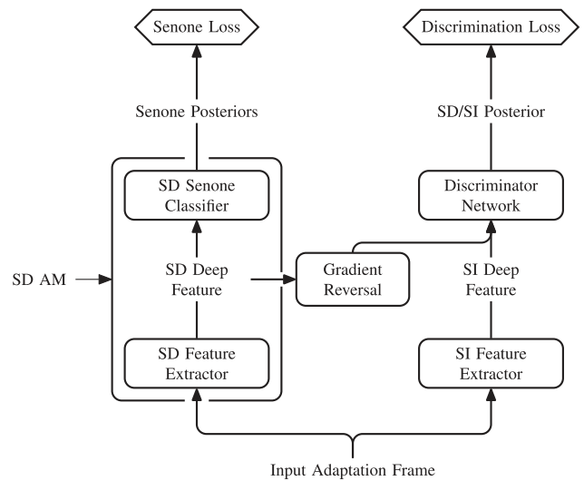
FIGURE 4. Adversarial speaker adaptation.
