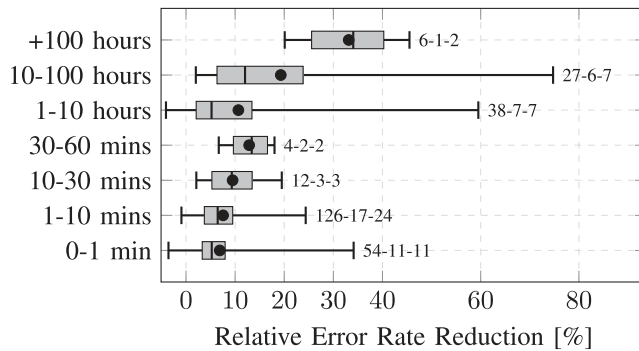
FIGURE 14. Comparison of adaptation results for different amount of adaptation data.
