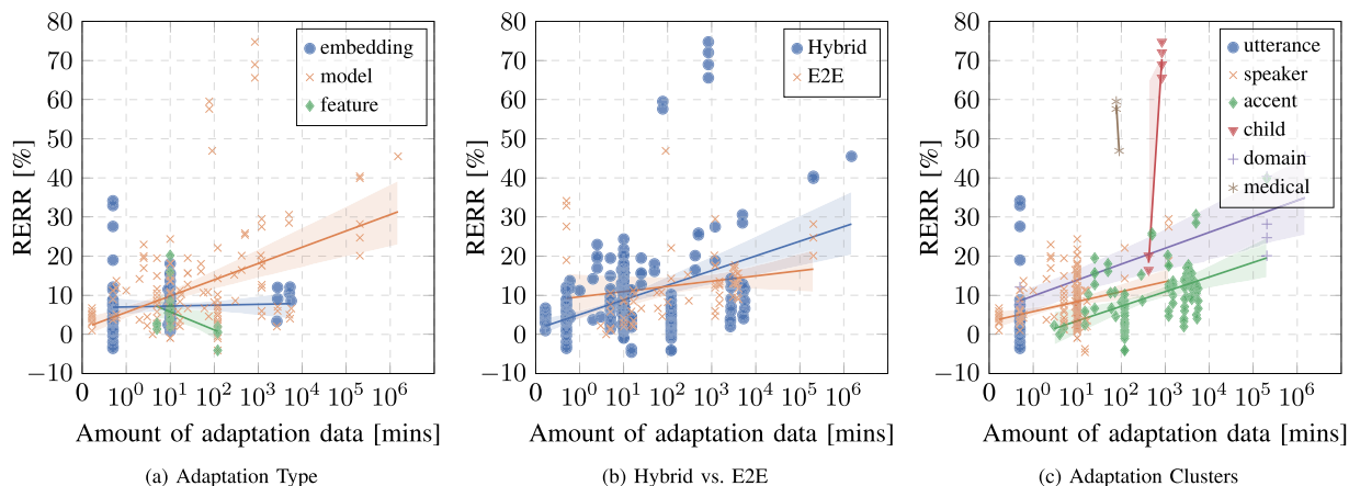
FIGURE 16. Regression analysis for the three major control variables.
