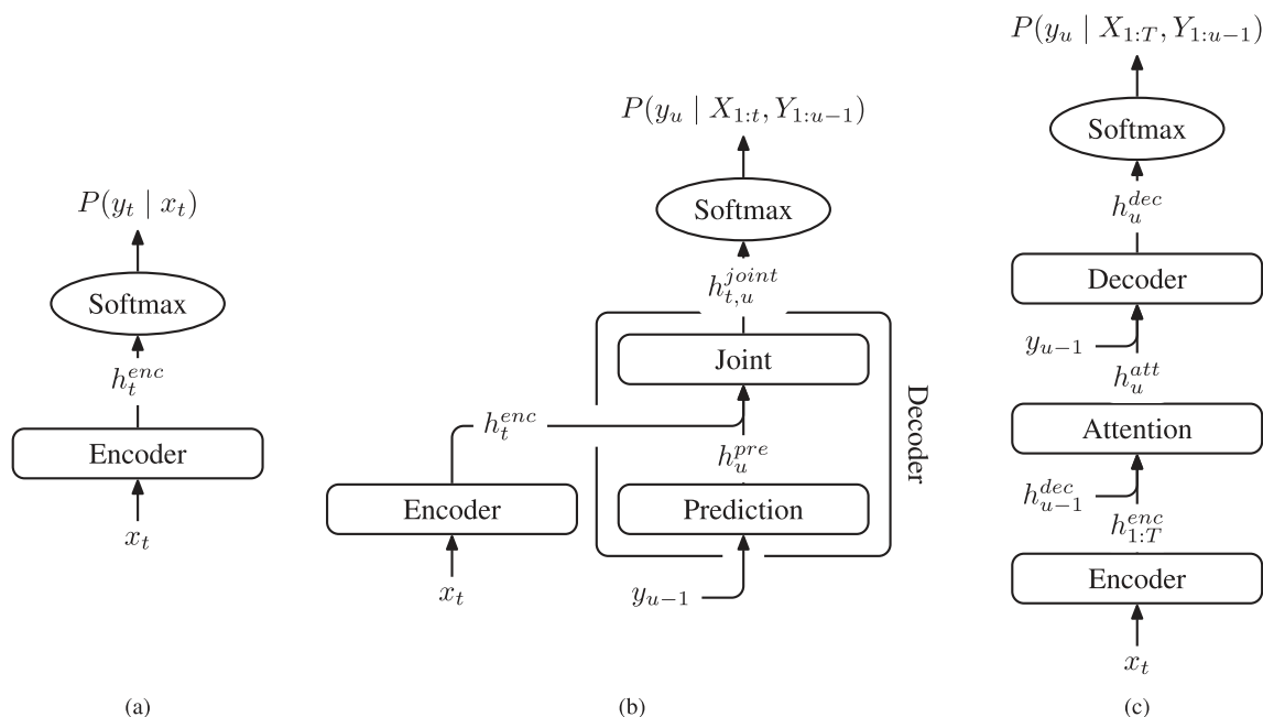
FIGURE 1. NN architectures used for hybrid NN/HMM and end-to-end (CTC, RNN-T, AED) speech recognition systems: (a) Scheme of NN architecture used for NN/HMM hybrid systems and for connectionist temporal classification (CTC); (b) architecture for the RNN Transducer (RNN-T); (c) architecture for attention based encoder-decoder (AED) end-to-end systems. Input acoustic feature vectors are denoted by x_t ; hidden layers are denoted by h_t , h_u and output labels by y_t , y_u depending on whether they are indexed by time t (in hybrid and CTC systems) or only by output label u (in parts of RNN-T and AED systems). In practice, the encoders use a wide temporal context as input, even the whole acoustic sequence in the case of most CTC and AED models.
