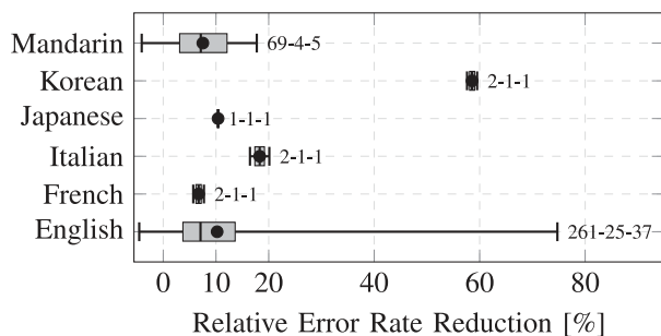
FIGURE 27. Adaptation gains for different languages.
