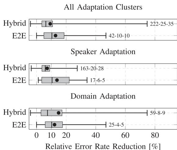
FIGURE 9. Comparison of adaptation results for hybrid and E2E systems.
