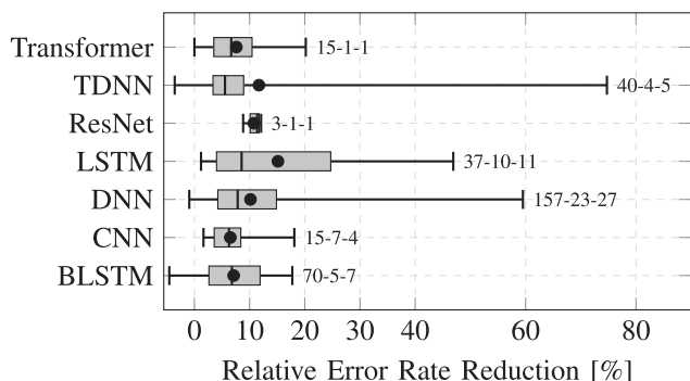
FIGURE 22. Comparison of adaptation results for different architectures.
