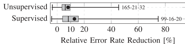
FIGURE 12. Comparison of adaptation results for supervision modes.
