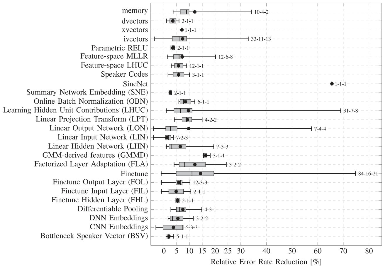
FIGURE 24. Comparison of adaptation results for the standalone techniques.
