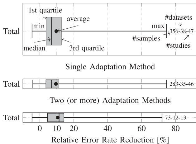
FIGURE 6. Aggregated summary of adaptation RERR from all studies (top), considering single method only (middle) and two or more methods stacked (bottom). The top graph is annotated to explain the information presented in each of the boxplot graphs in this section.
