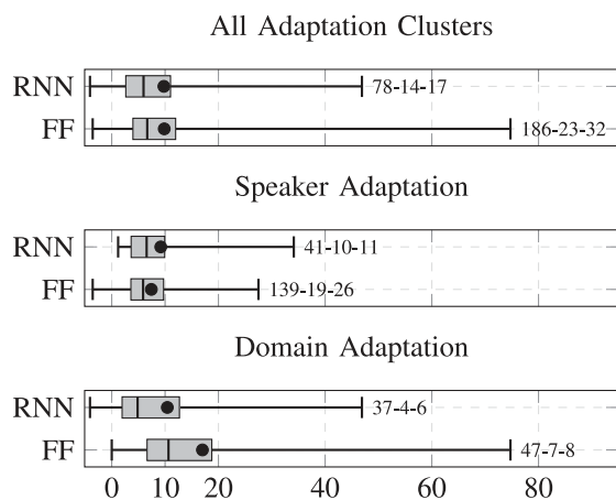
FIGURE 10. Comparison of adaptation results for FF and RNN architectures.
