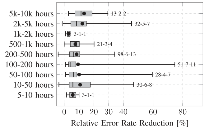
FIGURE 15. Comparison of adaptation results for acoustic models estimated from different amounts of training data.
