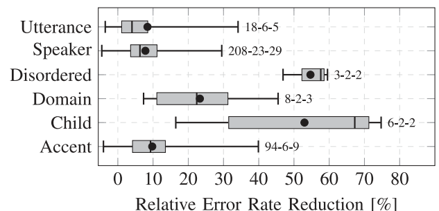
FIGURE 8. Adaptation results for different adaptation clusters.
