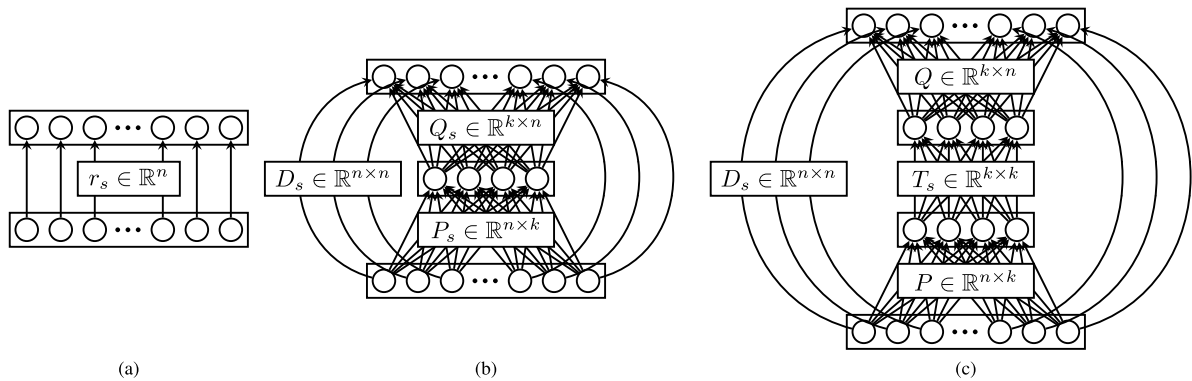
FIGURE 3. Structured transforms of an adaptation matrix A_s : (a) Learning Hidden Unit Contributions (LHUC) adapts only diagonal elements of the transformation matrix r_s = \text{diag}(A_s) ; (b) Low-Rank Plus Diagonal factorizes the adaptation matrix as A_s \approx D_s + P_s Q_s ; (c) Extended LRPD factorizes the adaptation matrix as A_s \approx D_s + P T_s Q .
