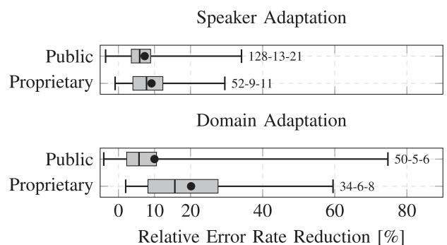
FIGURE 26. Performance of adaptation techniques as obtained on public and proprietary datasets.
