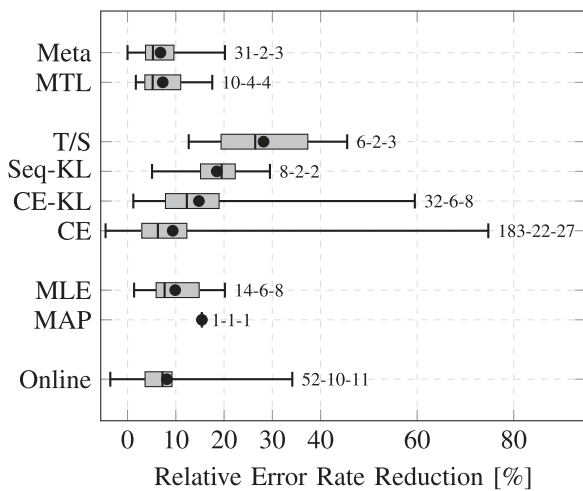
FIGURE 20. Comparison of results for different adaptation loss functions.
