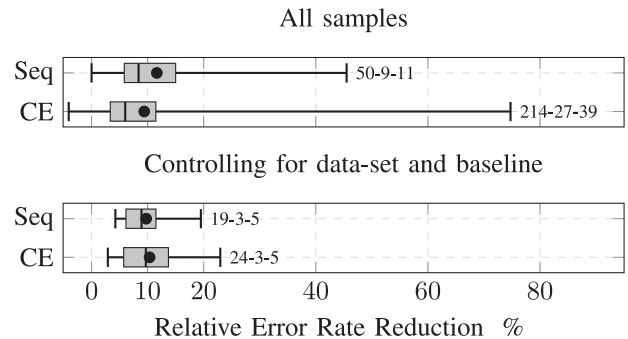
FIGURE 21. Comparison of adaptation results for acoustic models trained with CE and Sequence-level objectives.
