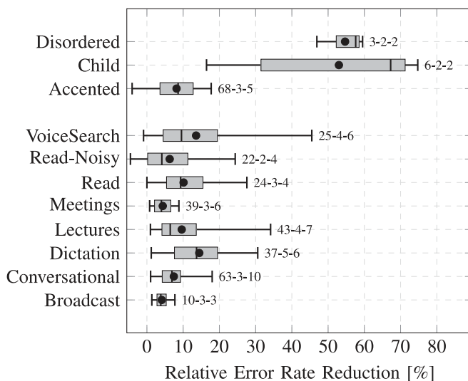
FIGURE 25. Comparison of adaptation results for different speech styles.
