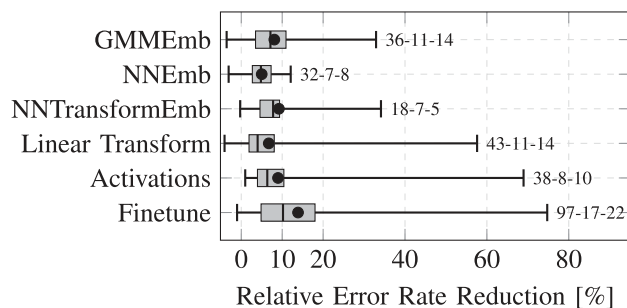
FIGURE 17. Comparison of results for different adaptation approaches.
