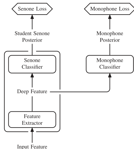
FIGURE 5. Multi-task learning speaker adaptation.
