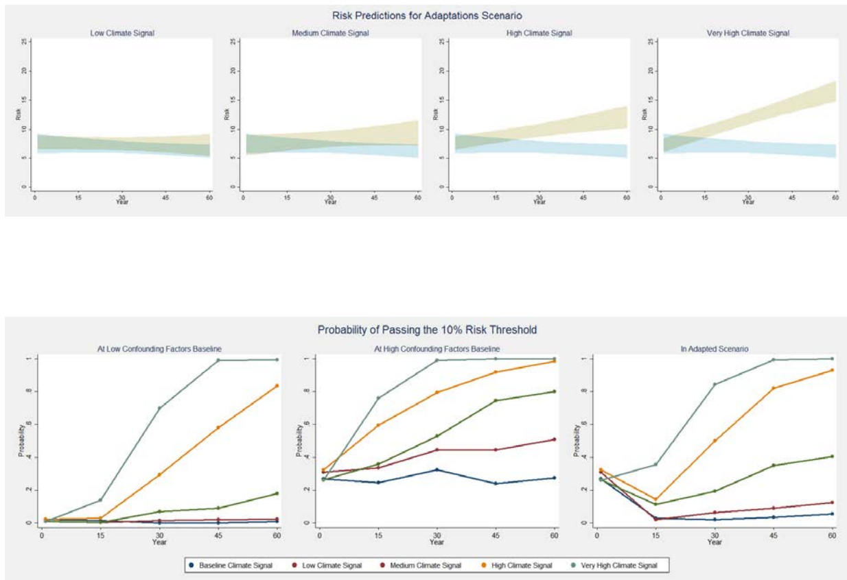
Figure 7: Sensitivity of risk over time. Probability of crossing the operative threshold of tolerable risk ( Y_t = 10 ) along any of the five scenarios at benchmark years in the future.
