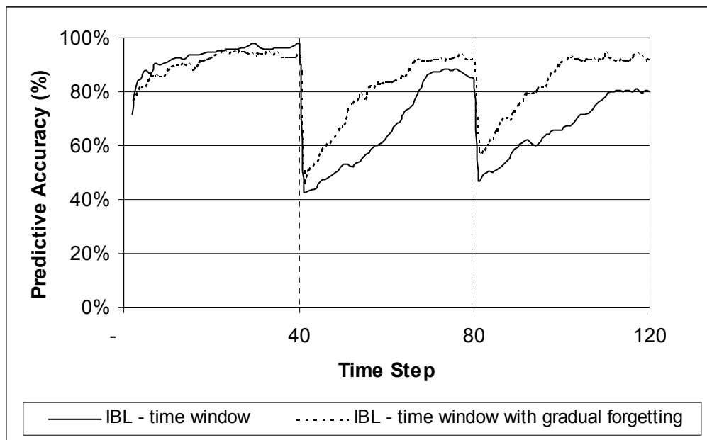
Figure 2. The STAGGER problem: The improvement in predictive accuracy when a gradual forgetting function is utilized in a time window.
