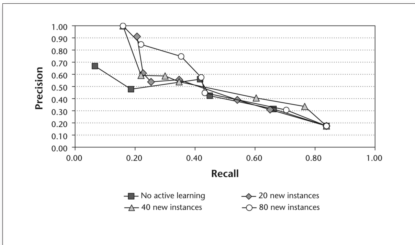
Figure 8. Results of Active Learning on the GameWinner Relation.
