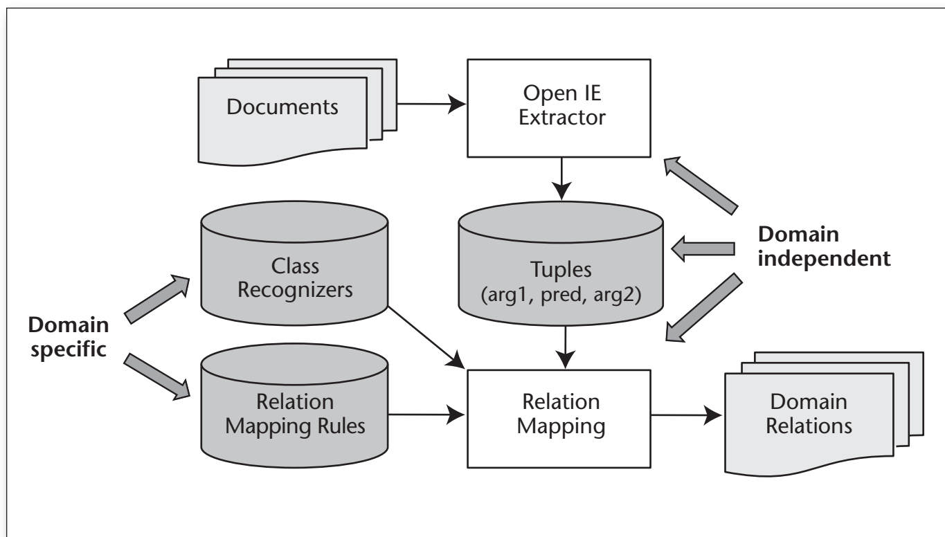
Figure 2. System Architecture.
