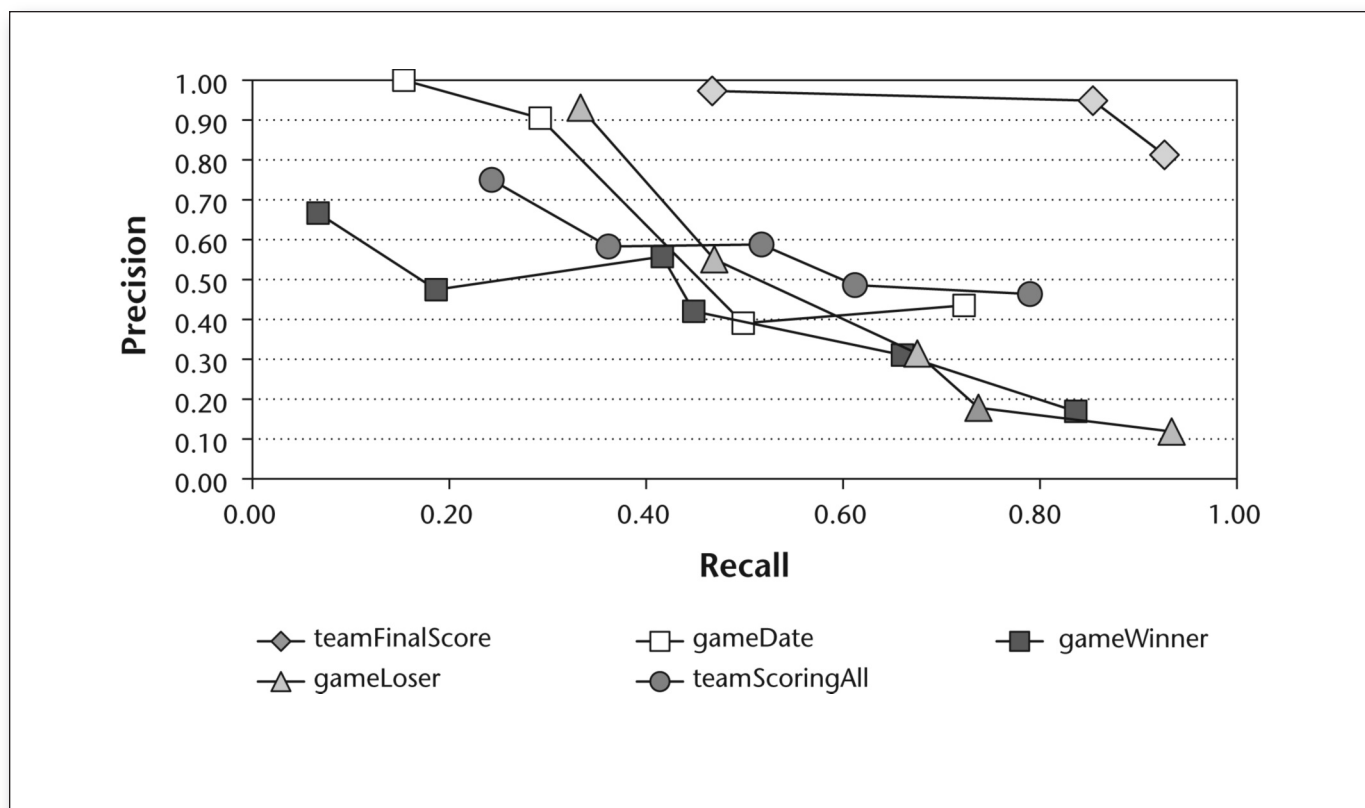
Figure 7. TEXTRUNNER Performance.
