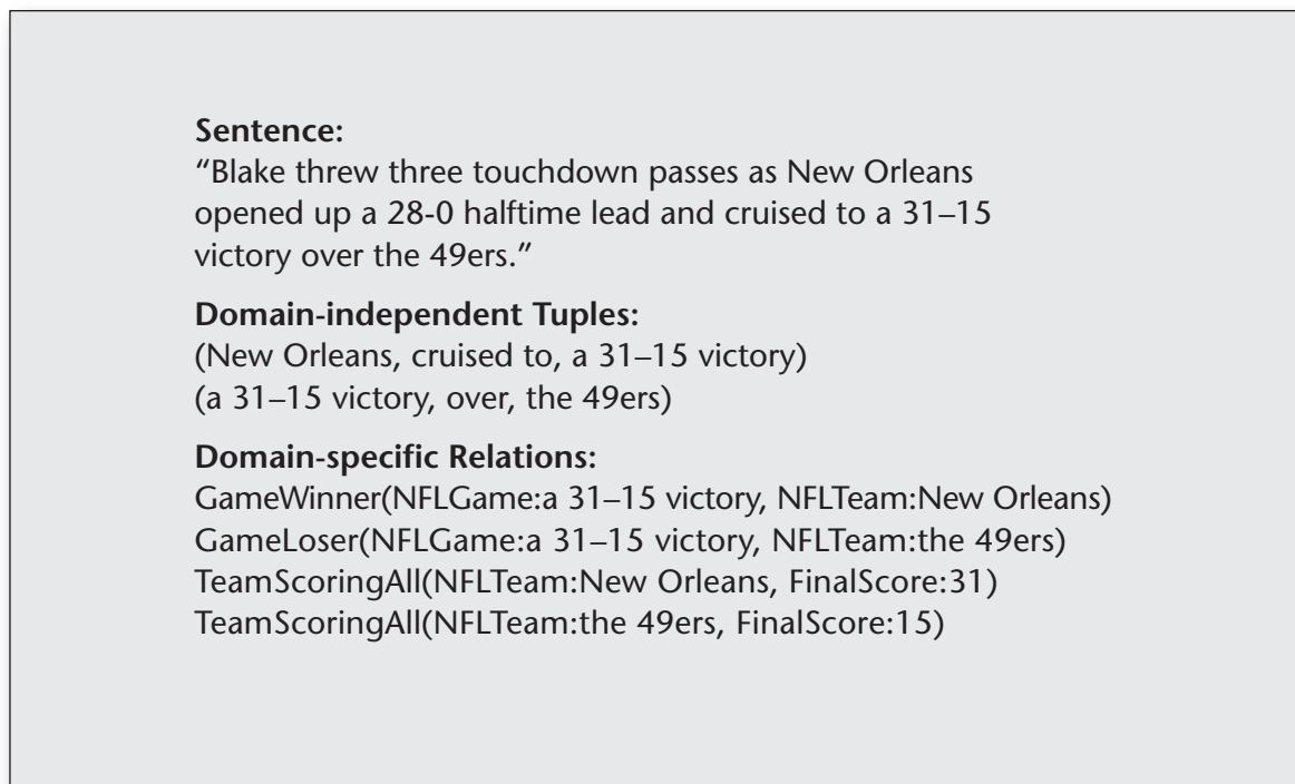
Figure 1. Desired Output for a Sample Sentence.
