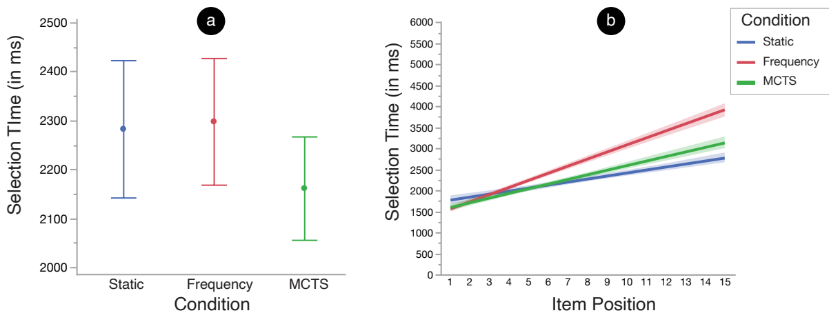
Figure 9: (a) The MCTS condition was associated with significantly lower selection time as compared to the two baselines. Vertical bars indicate 95% confidence intervals. (b) For items positioned lower in the menu, selection time in FREQUENCY increased more drastically than other conditions.
