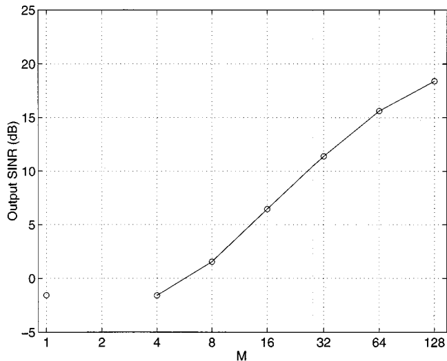
Fig. 15. Output SINR versus M ( \sigma_{D1}^2 = \sigma_{D2}^2 = 10 dB, \theta_{D1} = 0^\circ , \theta_{D2} = 20^\circ , \tau_D = 4T_S , \sigma_{I1}^2 = \sigma_{I2}^2 = 20 dB, \theta_{I1} = -20^\circ , \theta_{I2} = -60^\circ , \tau_I = 4T_S ).
