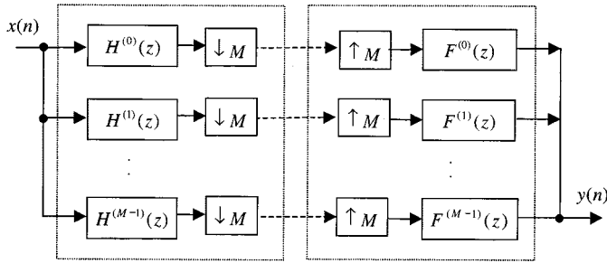
Fig. 3. Block diagram of a filter bank.
