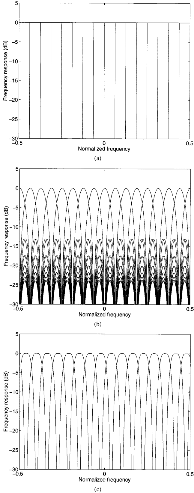
Fig. 5. Frequency response of different filter banks ( M = 16 ). (a) Ideal filter bank. (b) DFT filter bank. (c) Modified QMF bank.
