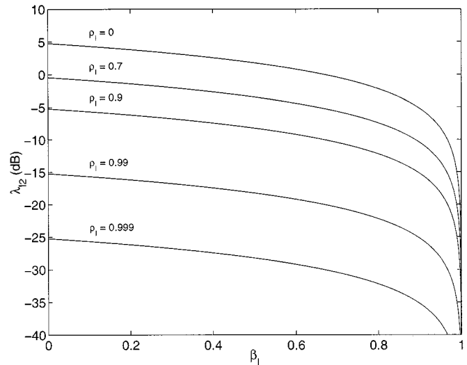
Fig. 2. \lambda_{I2} versus \rho_I and \beta_I .
