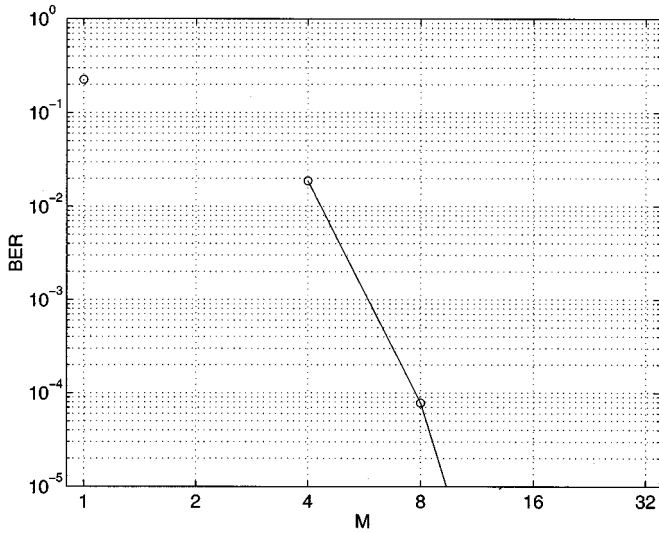
Fig. 13. BER versus M ( \sigma_{D1}^2 = \sigma_{D2}^2 = 10 dB, \theta_{D1} = 0^\circ , \theta_{D2} = 20^\circ , \tau_D = T_S , \sigma_{I1}^2 = \sigma_{I2}^2 = 20 dB, \theta_{I1} = -20^\circ , \theta_{I2} = -60^\circ , \tau_I = T_S ).
