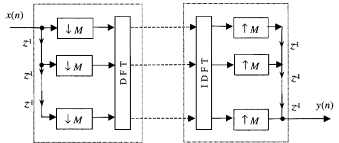
Fig. 4. Block diagram of a DFT filter bank.
