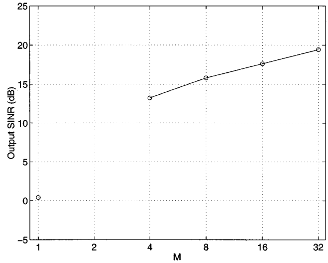
Fig. 11. Output SINR versus M ( \sigma_{D1}^2 = \sigma_{D2}^2 = \sigma_{D3}^2 = \sigma_{D4}^2 = 10 dB, \theta_{D1} = 0^\circ , \theta_{D2} = 20^\circ , \theta_{D3} = -20^\circ , \theta_{D4} = -60^\circ , \tau_2 = T_S , \tau_3 = 2T_S , \tau_4 = 3T_S ).
