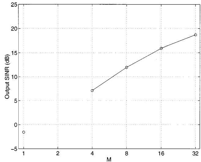
Fig. 12. Output SINR versus M ( \sigma_{D1}^2 = \sigma_{D2}^2 = 10 dB, \theta_{D1} = 0^\circ , \theta_{D2} = 20^\circ , \tau_D = T_S , \sigma_{I1}^2 = \sigma_{I2}^2 = 20 dB, \theta_{I1} = -20^\circ , \theta_{I2} = -60^\circ , \tau_I = T_S ).
