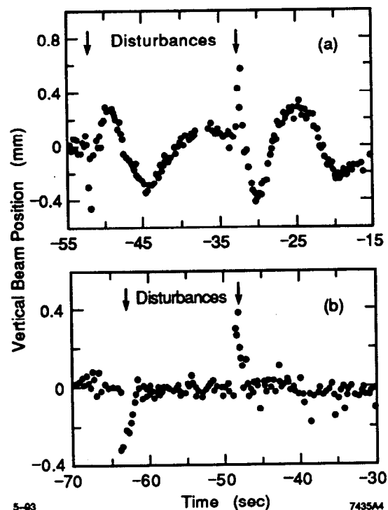
5-03 743544 Figure 3. Response of a chain of six feedback loops to a sudden disturbance in the incoming beam. In part (a) adaptive noise cancelling is off so there is a ringing caused by the over correction of many loops. In part (b) adaptive noise cancelling is on, so the whole chain of loops responds like a single loop. In fact, the first loop did all the work to correct the beam and the downstream loops did virtually nothing.
