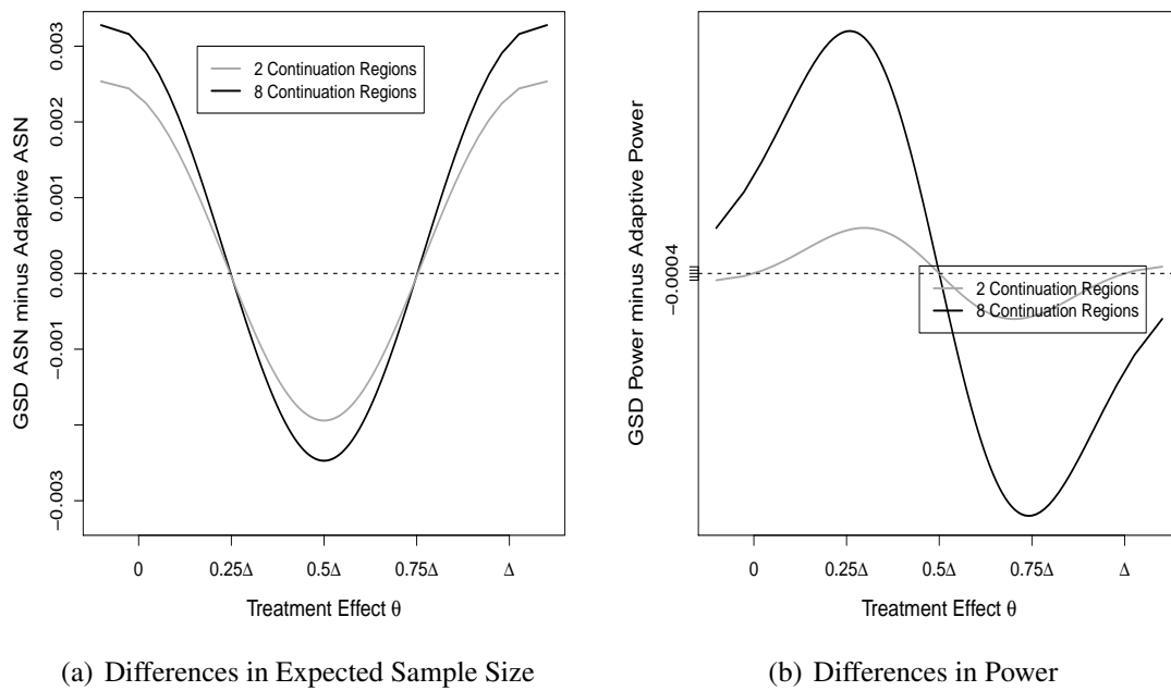
Figure 3: Comparison of the group sequential design to two representative optimal adaptive designs with respect to power and ASN across a range of plausible treatment effects. Differences between the group sequential and adaptive operating characteristics are shown on the y-axes. ASN differences are in units of the fixed sample size n . The dotted line indicates equality.
