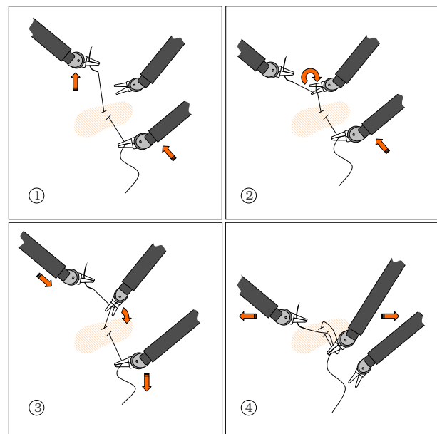
Fig. 3. Knot-Tying Procedure: After piercing, the needle with the thread is pulled out of the tissue with the left gripper (1) and winded about the right gripper (2). During this procedure, the loose end of the thread is retained by an assistant. This facilitates grasping of the end by the right gripper (3). Finally, the end of the thread is pulled through the loop around the right gripper in order to finalize the knot (4).
