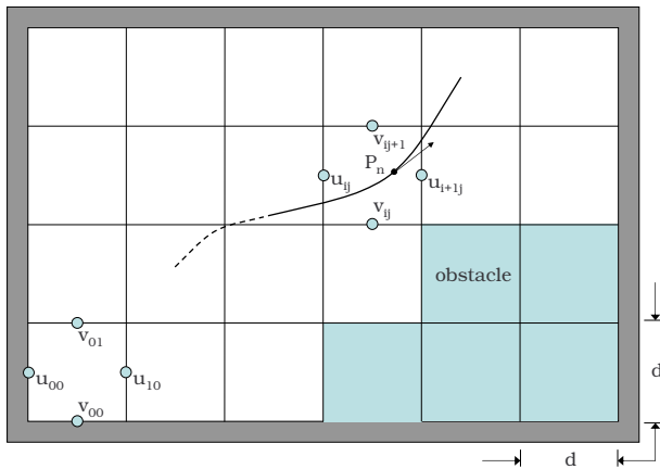
Fig. 6. Fluid simulation: The area of interest is discretized into equally sized cells. For clarity reasons this picture shows only a limited number of cells which would be too coarse for practical use - the actual implementation usually works on a grid of at least 50 \times 50 cells. Evaluation of velocities is not centered within a cell, but distributed on a staggered grid in order to assure numeric stability.
