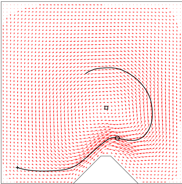
Fig. 8. Obstacles: The same primitive as depicted in fig. 7 adapted to an obstacle. At each time step the obstacle is inserted into the raster and simulation is continued under the new circumstances. Additionally, this leads to a shift of the fixture point (marked with a quad) and therefore will also have influence on other primitives (e.g. the movement of the second gripper). Note that the shape of the obstacle is improved for illustration - the real shape used for simulation is discretized with quads at cell level.
