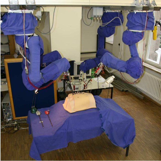
Fig. 2. Hardware Setup: Four ceiling mounted robots can be equipped with either a stereoscopic endoscope or different surgical instruments. Instruments are augmented with force sensors. In-output is accomplished at a master console, comprising two 6Dof force feedback devices
