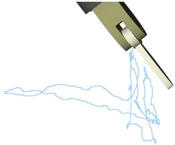
Fig. 4. Knot-Tying Trajectory: Visualization of the trajectory of the left gripper during knot-tying. For clarity reasons, the right gripper and its trajectory are hidden. The image was produced with the 3D planning and recording software of our system.
