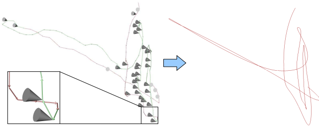
Fig. 5. Spline approximation: Significant points are selected from the recorded trajectory (cones on left image). These points serve as breakpoints for a spline approximation of the trajectory (right image). Note that human tremor is annihilated while all significant edges are preserved
