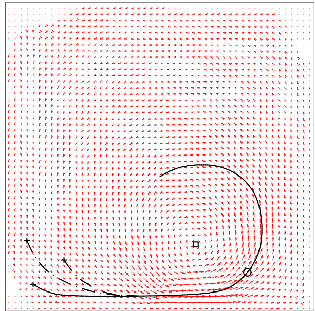
Fig. 7. Flow visualization: Fluid simulation of the winding primitive. The vector field is a snapshot at the time step, where the particle (i.e. the gripper) is at the position marked with a circle. Note that the depicted trajectories are overlays just for illustration and the vector field looks different for all other time steps. Therefore, parts of the depicted trajectories might be contradictory to the vector field which is only valid for this particular time step.
