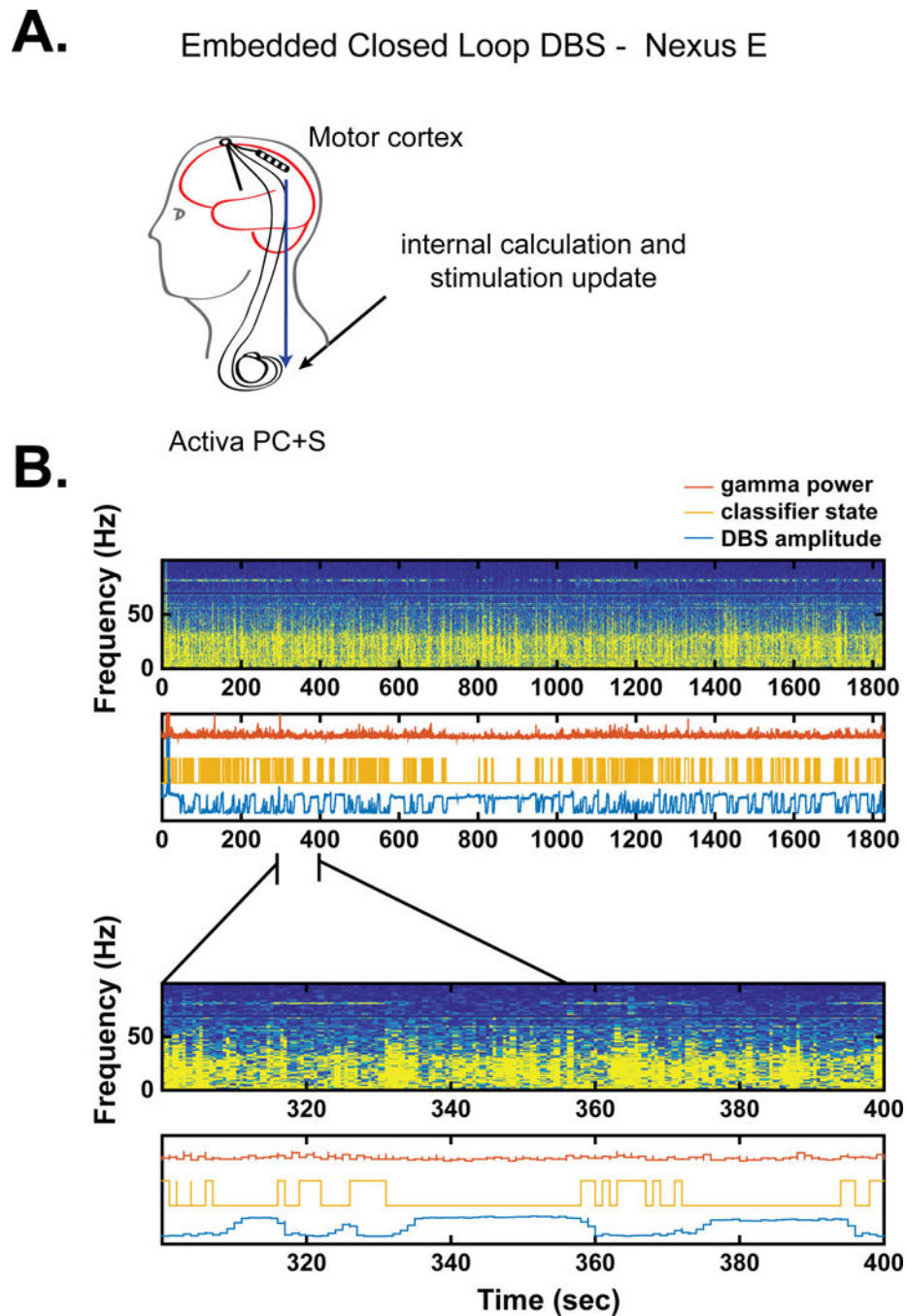
Figure 4. Adaptive DBS utilizing Activa PC+S with fully embedded control (Nexus E), from Patient 1. A. Schematic of fully embedded control. B. Neural data, classifier state, and stimulation state during adaptive DBS. Panel format same as Figure 2. Note the more frequent transitions in the classifier compared to Nexus D3. This is likely because the Nexus E algorithm did not incorporate any smoothing of the signal, whereas Nexus D3 averaged the gamma signal over time before triggering a change in stimulation. This type of smoothing was not supported by Nexus E.
