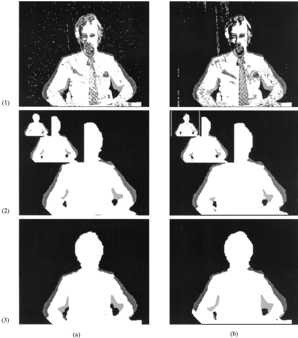
Fig. 9. Localization for Trevor White sequence: (a) histograms analysis with mixture of Gaussian distributions; (b) histograms analysis with mixture of uniform distributions; (1) maximum-likelihood detection maps; (2) detection maps with ICM algorithm and multiscaling in label and data spaces; (3) detection maps with HCF algorithm and multiscaling in label space.
