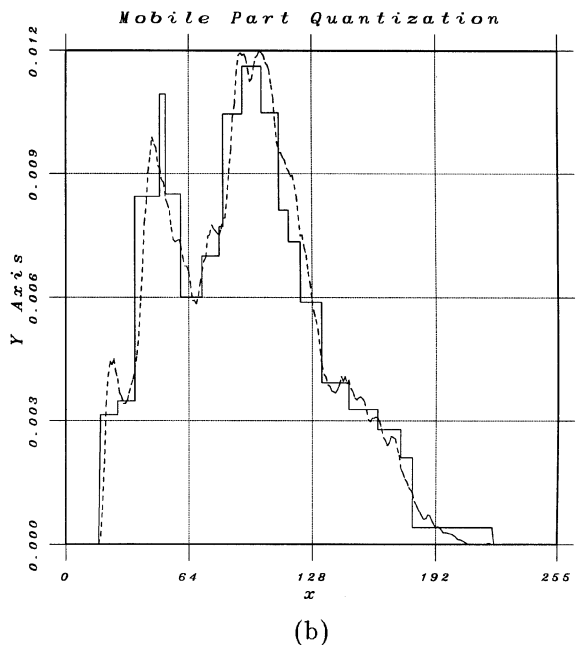
Fig. 7. Approach with piecewise uniform distributions: Trevor White sequence: (a) static part; (b) mobile part.
