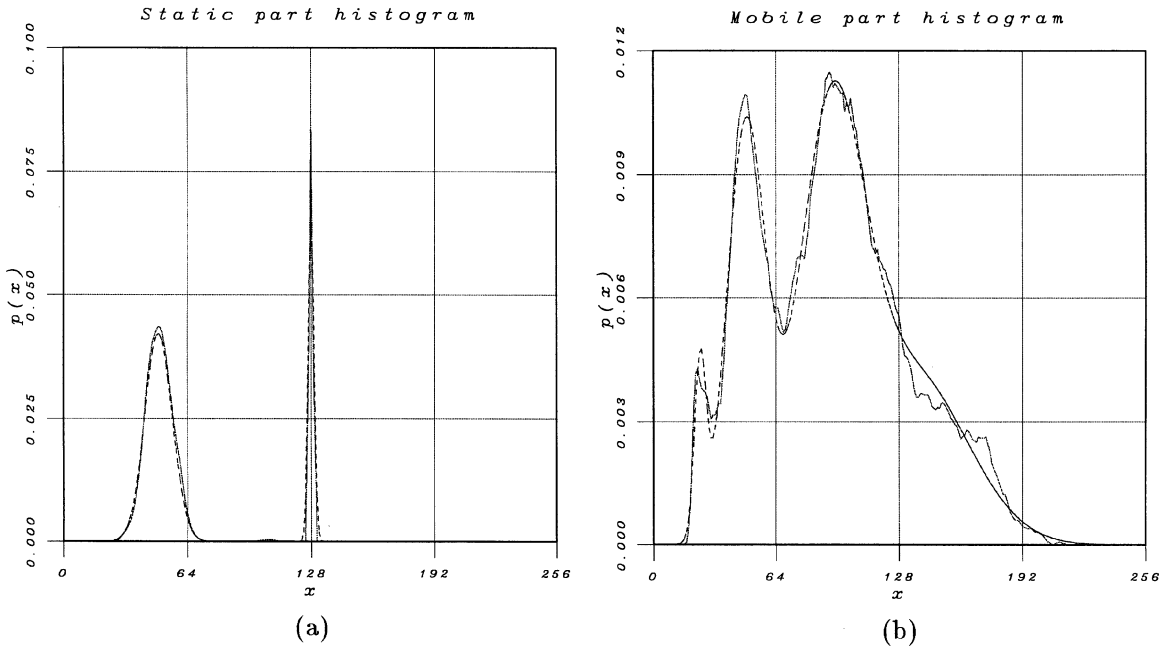
Fig. 8. Approach with mixture of Gaussian distributions: Trevor White sequence: (a) static part; (b) mobile part.
