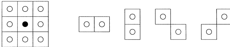
Fig. 1. Second-order neighborhood: a possible choice of effective cliques.
