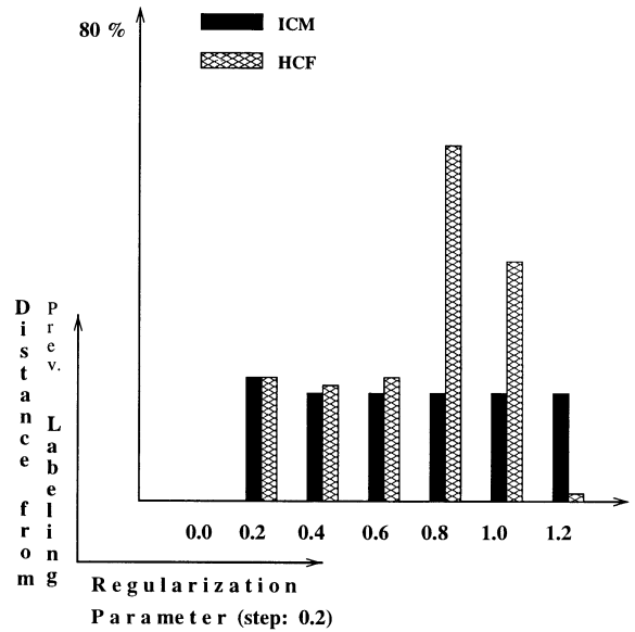
Fig. 13. Sensitivity on regularization for ICM, HCF.
