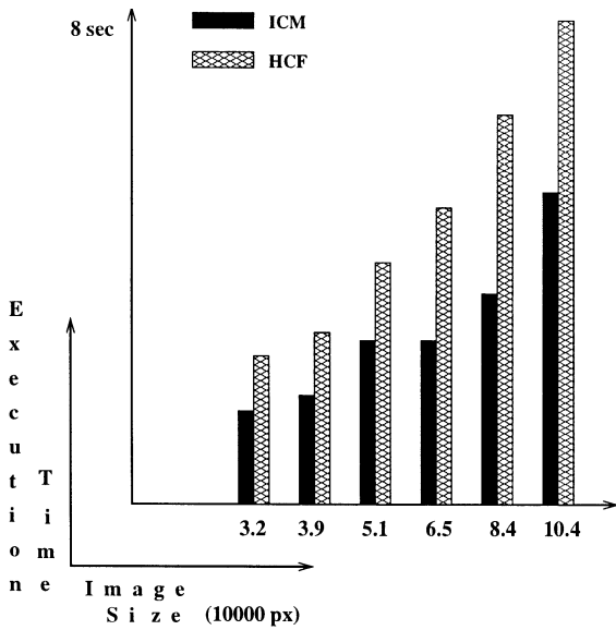
Fig. 12. Computational cost for ICM, HCF.
