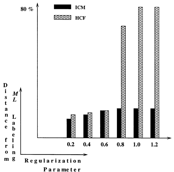
Fig. 14. Dependency from Maximum-likelihood labeling for ICM, HCF.
