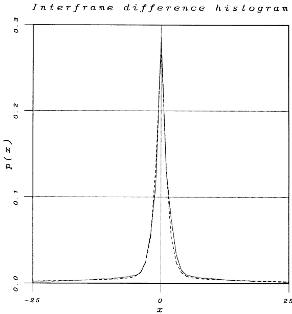
Fig. 4. Mixture decomposition for inter-frame difference for Trevor White.
