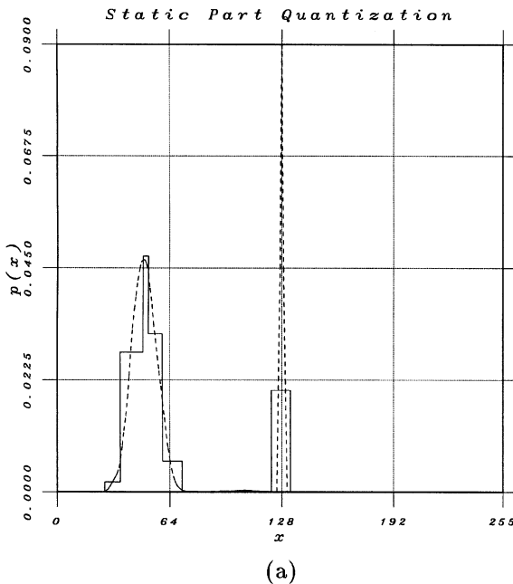
Fig. 7. Approach with piecewise uniform distributions: Trevor White sequence: (a) static part; (b) mobile part.
