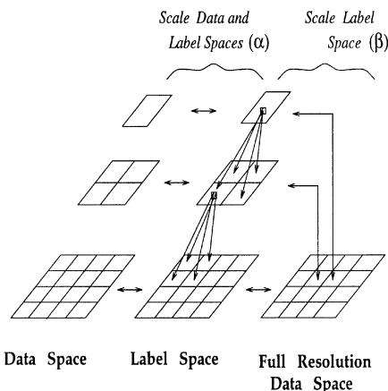
Fig. 2. Multiscale techniques: (a) multiresolution; (b) multigrid.
