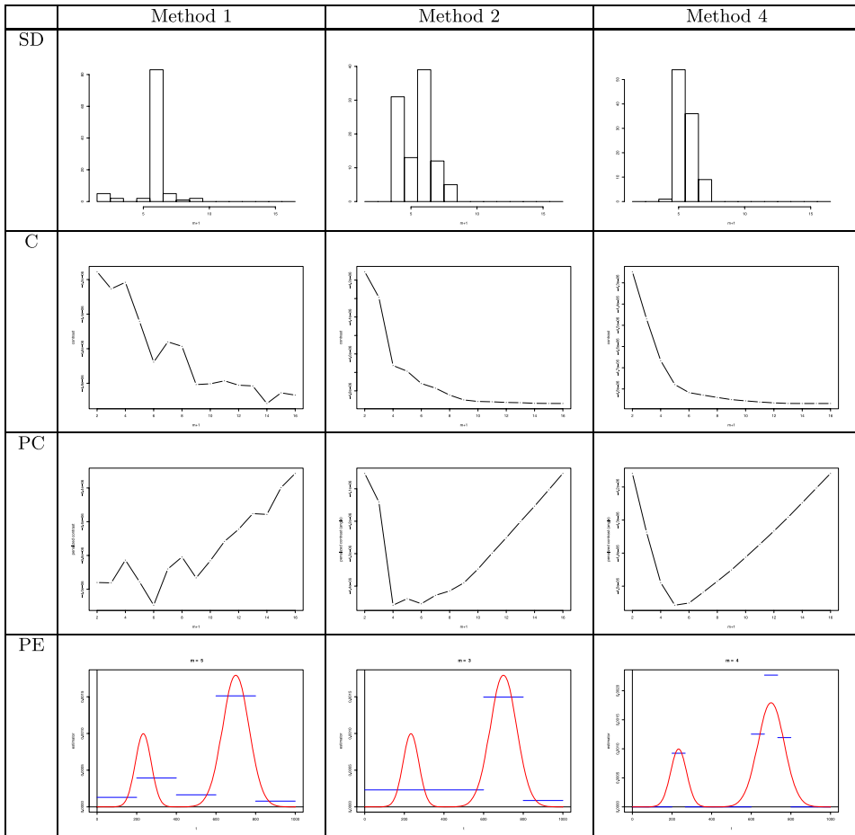
FIG. 9. Histogram of the selected dimension over 100 simulations (SD). Contrast (C) and penalized contrast (PC) as a function of the dimension for the three favorite methods on one simulation with T = 500,000 , \nu = 0.001 and h = f_3 . The chosen estimators (PE) are in blue whereas the function h = f_3 is in red.
