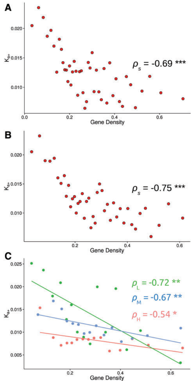
FIG. 2. Relationship between K_{a+} in the y axis and the gene density (coding sequences sites /100,000 sites) in the x axis: (A) using the whole data set, (B) excluding immune response and testes related genes and (C) splitting the data set into three Fop groups. Genes belonging to the high (H) group are in red, medium (M) genes are in blue, and low (L) genes are in green. Each data point has been estimated binning genes. The number of genes, the average gene density, Fop , and K_{a+} estimate for each bin can be consulted in the supplementary table S4 , Supplementary Material online. \rho_s : Spearman's rank correlation coefficient, with significance denoted by asterisks (***) < 0.001 ; (**) < 0.01 ; (*) < 0.05 ). The lines are least-squares regressions but should be regarded only as indicative, in view of the binning of the data.
