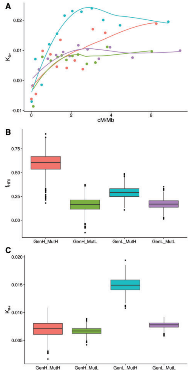
FIG. 4. (A) Relationship between K_{a+} in the y axis and the rate of recombination (cM/Mb) in the x axis for each gene category; the lines are LOESS regressions. (B) Bootstrap f_{\text{HRi}} values and (C) bootstrap K_{a+} values for each gene category, respectively. Each data point has been estimated binning 128 genes according to their gene density, mutation rate ( K_{4,1} ) and recombination rate (in cM/Mb). GenH-MutH genes are in red, GenH-MutL genes are in green, GenL-MutH genes are in blue, and GenL-MutL genes are in purple; see the full description of these gene categories in the main text.
