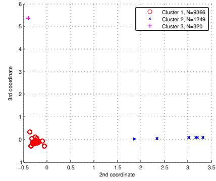
Figure 3. Resource 1, diffusion map.
