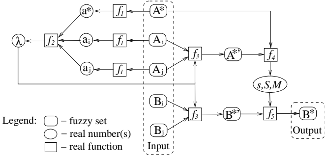
Fig. 2. Transformation-based interpolation
