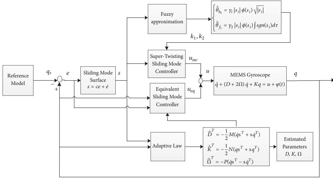
FIGURE 2: Block diagram of the adaptive fuzzy super-twisting sliding mode control.
