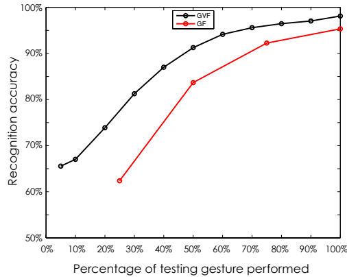
Fig. 5. Early recognition rates obtained with GVF and GF (for a more complete study of the GF evaluation on the same database, please refer to [Zamborlin et al. 2014])
