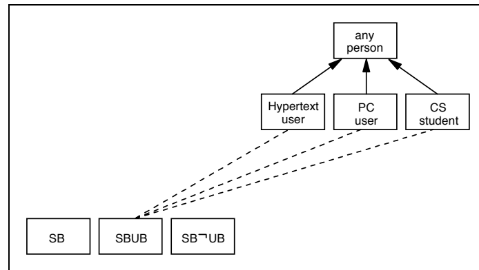
Fig. 2: Partition Hierarchy in SB-PART
