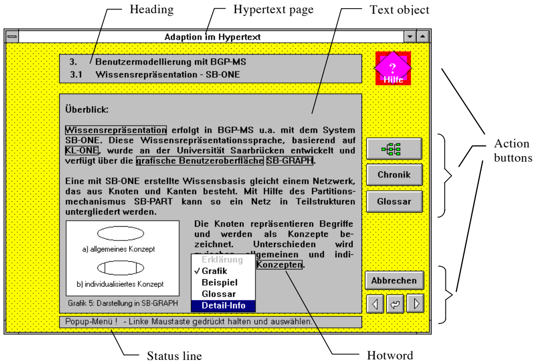
Fig. 4: Selecting additional information on a hotword
