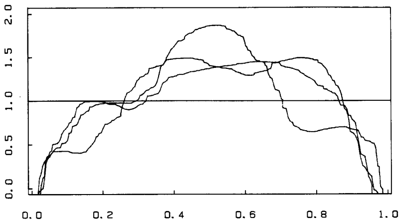
FIG. 1. Three \hat{J} 's with Gaussian errors.
