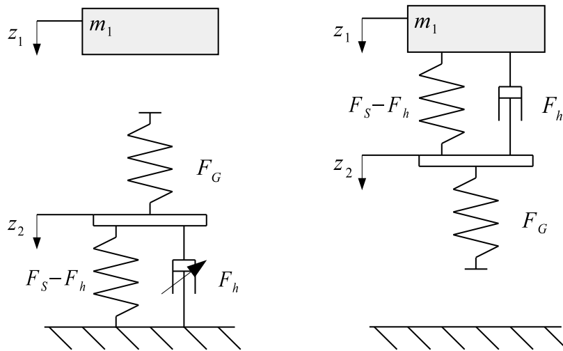
Figure 18: Comparison of schemes of testing stands: (left) lab-scale; (right) full-scale
