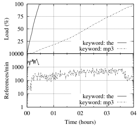
Fig. 3. Load and publishing frequency over time registered by our instrumented client.
