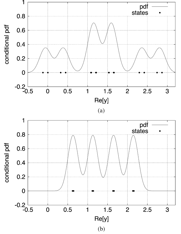
Fig. 4. Conditional pdfs given b_1(k) = +1 and subsets \mathcal{Y}_R^{(+)}(\mathbf{w}) of the MMSE and MBER beamformers for SNR = 15 dB and SIR_i = -6 dB for i = 2, 3, 4, 5 : (a) MMSE and (b) MBER.
