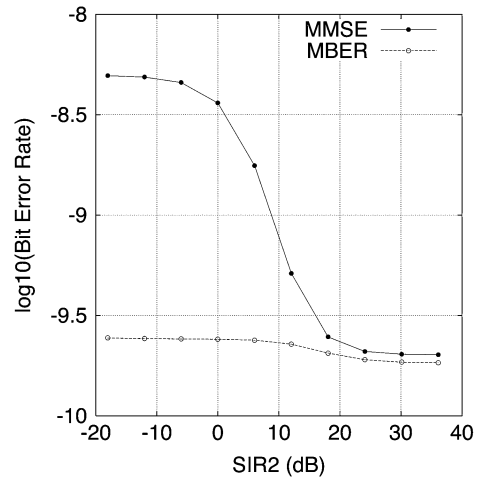
Fig. 2. Influence of near-far effect on BER performance of the MMSE and MBER beamformers for SNR = 10 dB and \text{SIR}_i = 24 dB for i = 3, 4, 5 .
