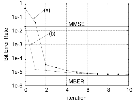
Fig. 5. Convergence rate of the block-data-based gradient adaptive MBER algorithm of Section IV-A for a block size of K = 200 under the conditions SNR = 10 dB, SIR_2 = SIR_5 = -6 dB, and SIR_3 = SIR_4 = 0 dB. (a) \mathbf{w}(0) = [0.1 + j0.001 + j0.0]^T , \mu = 0.8 and \rho_n^2 = 2\sigma_n^2 = 0.1 . (b) \mathbf{w}(0) = \mathbf{w}_{MMSE} , \mu = 0.5 and \rho_n^2 = 2\sigma_n^2 = 0.1 .
