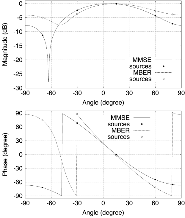
Fig. 3. Comparison of MMSE and MBER beam patterns for SNR = 10 dB and SIR_i = 0 dB for i = 2, 3, 4, 5 .
