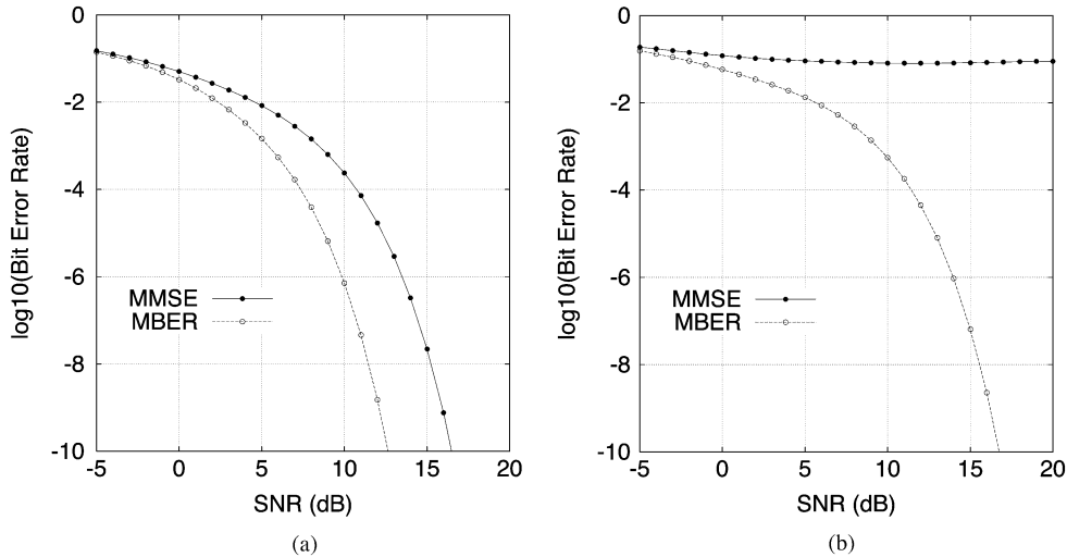
Fig. 1. Comparison of the BER performance of the MMSE and MBER beamformers: (a) \text{SIR}_i = 0 dB for i = 2, 3, 4, 5 and (b) \text{SIR}_i = -6 dB for i = 2, 3, 4, 5 .
