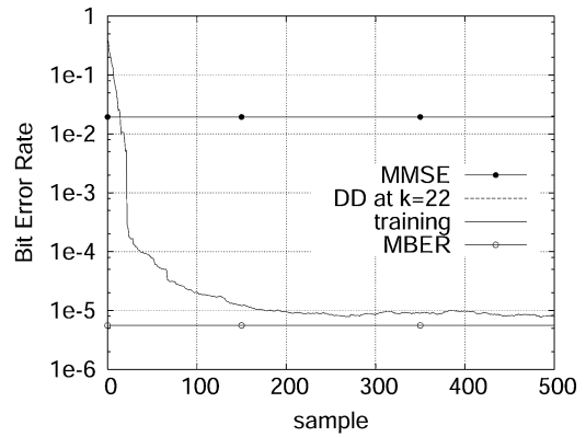
Fig. 7. Learning curves of the stochastic gradient adaptive MBER algorithm of Section IV-B averaged over 20 randomly chosen uniformly distributed initial weight values \mathbf{w}(0) . SNR = 10 dB, SIR_2 = SIR_5 = -6 dB, and SIR_3 = SIR_4 = 0 dB. DD denotes decision-directed adaptation in which b_1(k) is substituted by its estimate \hat{b}_1(k) . Note that the performance curves based on DD and explicit training are indistinguishable. Furthermore, we had \rho_n^2 = 4\sigma_n^2 = 0.2 and \mu = 0.2 for the first 25 samples, reducing the step size to \mu = 0.02 afterwards.
