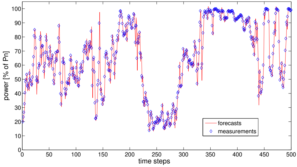
FIGURE 4: Time-series of normalized power generation at Nysted (both measurements and one-step ahead predictions) over an arbitrarily chosen episode.
