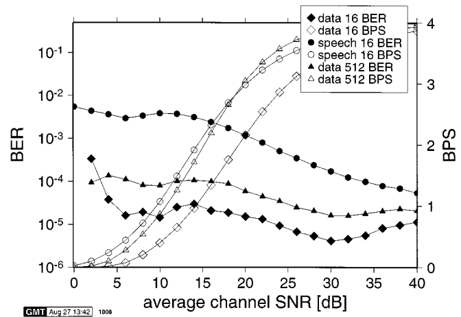
Fig. 4. BER and throughput performance of the 16 subband 512 subcarrier switching level adaptive OFDM modem employing BPSK, QPSK, 16-QAM and “no transmission” over the Rayleigh-fading time dispersive channel of Fig. 3.
