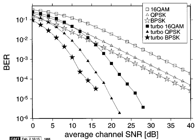
Fig. 12. BER performance of the 512-subcarrier OFDM modem in the fading time-dispersive channel of Fig. 3 for both uncoded and half-rate turbo-coded transmission, using 8-iteration turbo decoding, 1000-bit random interleaver and a constraint length of 3.
