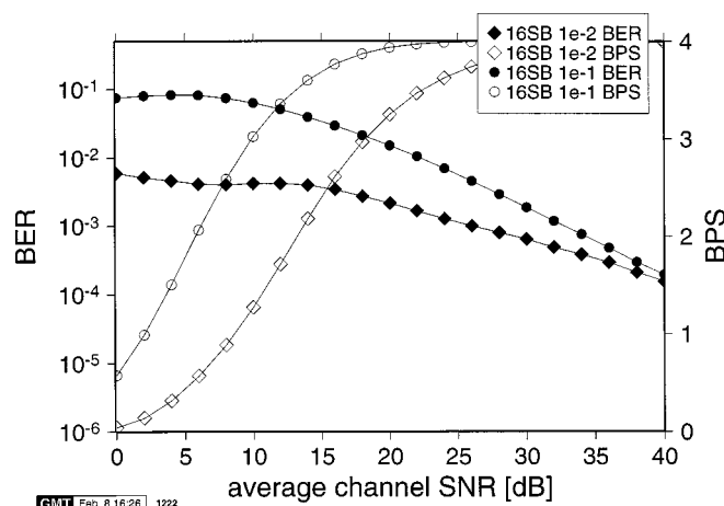
Fig. 5. BER and throughput performance of the 16 subband 512 subcarrier BER estimator adaptive OFDM modem employing BPSK, QPSK, 16-QAM and “no transmission” over the Rayleigh fading time dispersive channel of Fig. 3.
