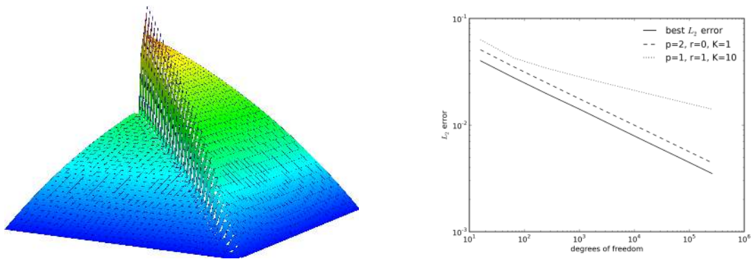
FIGURE 2. Left: solution for the model problem (6.1) on a uniform grid for the spaces X_h = \mathcal{P}_{1, \mathcal{T}_h} and Z_h = \mathcal{P}_{2, \mathcal{T}_h} \cap C(D) . Right: doubly logarithmic plot of the true errors for different test spaces Z_h . Here we vary the polynomial degree p , the additional refinements r and the number of iterations K . For reference we included the error of the best L_2 approximation to the solution u from X_h .
