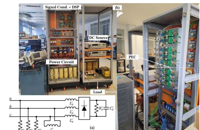
FIGURE 12. Experimental prototype: a) Unbalanced nonlinear load used to obtain experimental results; b) Picture of the prototype used to experimental validation of the proposed approach.
