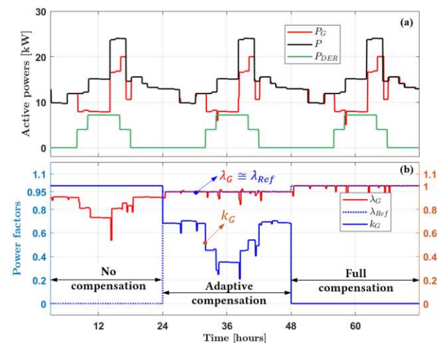
FIGURE 10. Real case study: multifunctional grid-connected inverter performance under time varying load demand condition and PV generation. (a) active powers, (b) power factors and compensation coefficient.
