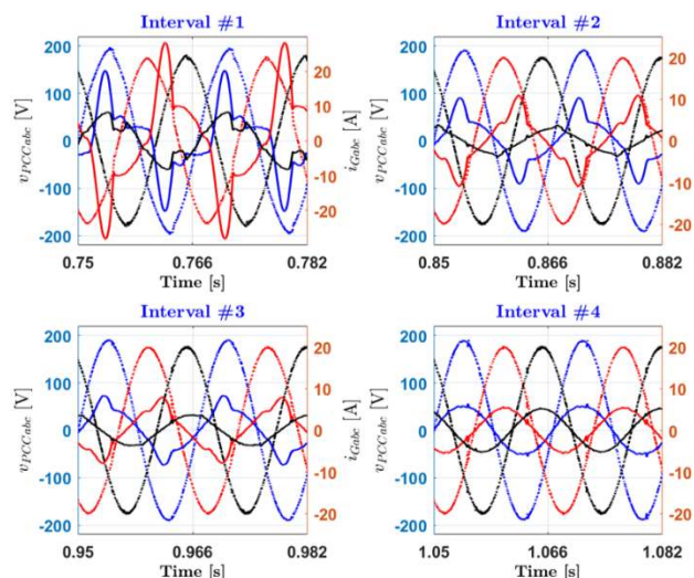
FIGURE 7. Detailed view of the PCC voltages and grid currents waveforms considering asymmetrical sinusoidal grid voltage condition.
