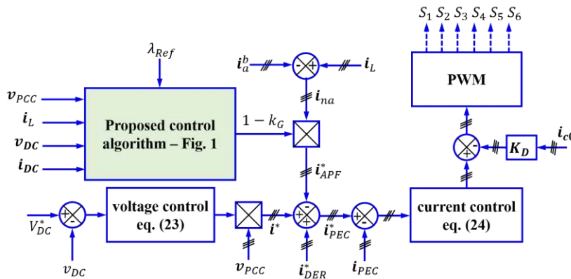
FIGURE 2. Proposed reference signal generator under time varying load conditions and intermittent nature of renewable generation.
