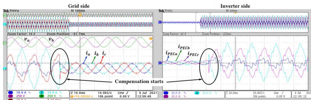
FIGURE 15. Dynamic response of grid and inverter currents due to a step change in power factor reference.
