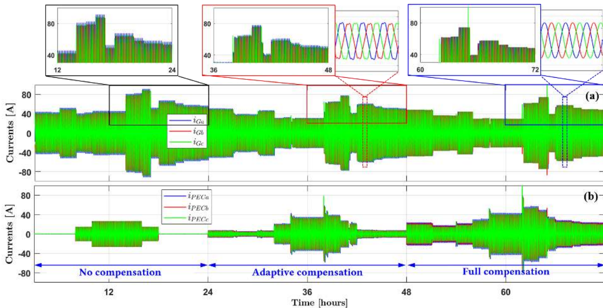
FIGURE 11. Real case study: time behavior of the multifunctional grid-connected inverter under time varying load demand condition and PV generation. (a) grid currents, (b) converter currents.
