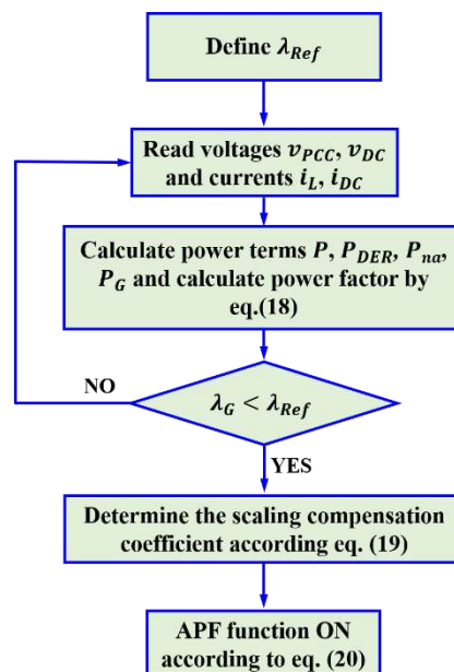
FIGURE 1. Flowchart of the proposed adaptable power factor compensation algorithm for time varying load conditions and intermittent nature of renewable generation.
