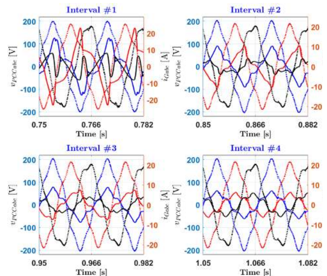
FIGURE 9. Detailed view of the PCC voltages and grid currents waveforms considering asymmetrical distorted grid voltage condition.
