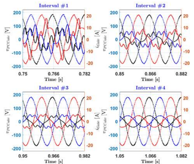
FIGURE 5. Detailed view of the PCC voltages and grid currents waveforms considering symmetrical sinusoidal grid voltages condition.
